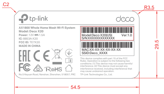
标贴尺寸: 54.5*29.5mm ±0.2
