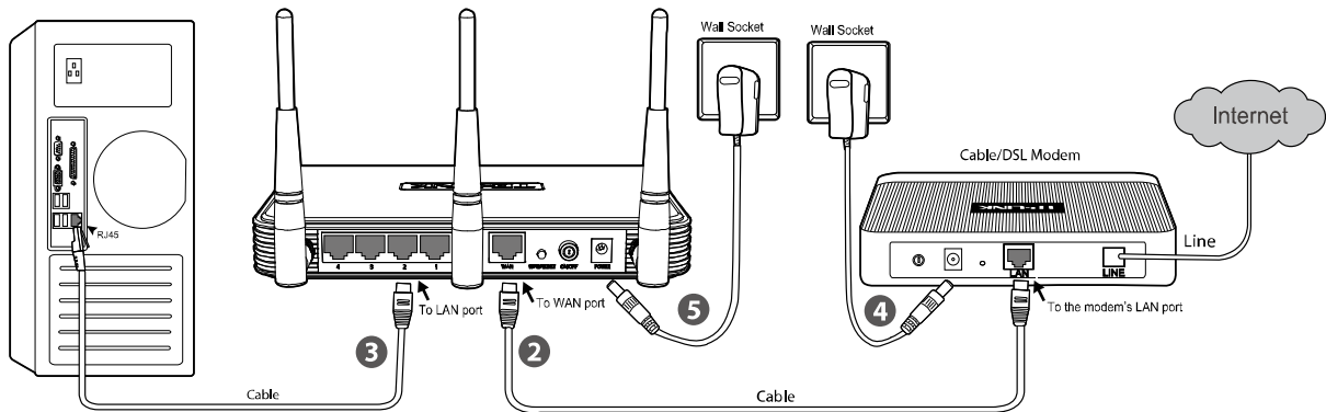
Figure 2-1 Hardware Installation of the TL-WR941ND 300Mbps Wireless N Router
