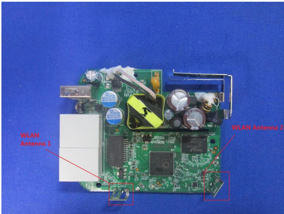
(3) EUT Photo Motherboard
