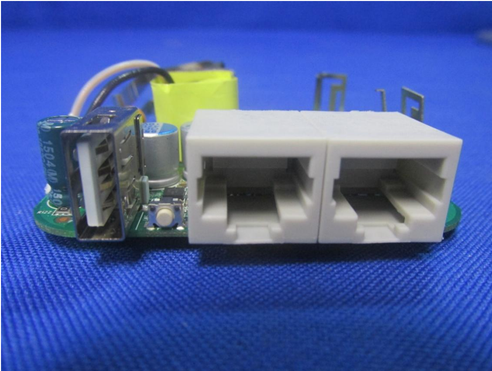
(5) EUT Photo Motherboard
