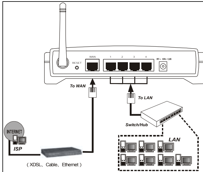
Figure 3-1 Hardware Installation of the TL-WR641G 108Mbps Wireless Router
