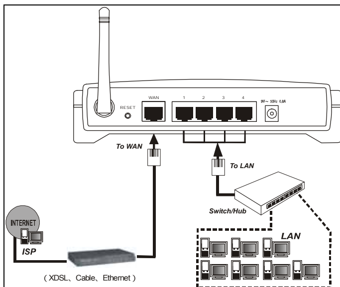
Figure 3-1 Hardware Installation of the TL-WR541G 54Mbps Wireless Router
