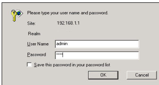
Figure 4-4 Login Windows
