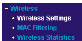
Figure 5-9: Wireless menu
