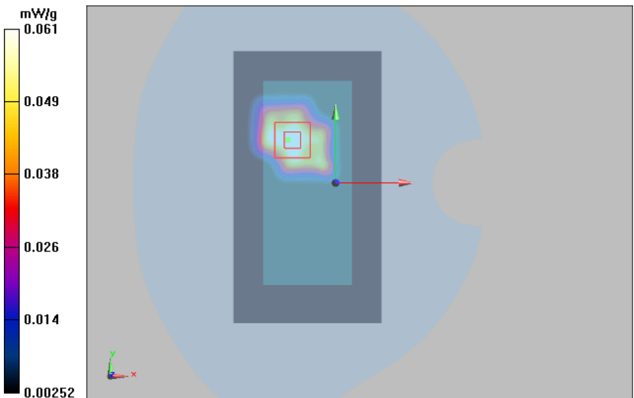
Figure 13 802.11g Chain 2 Channel 1
