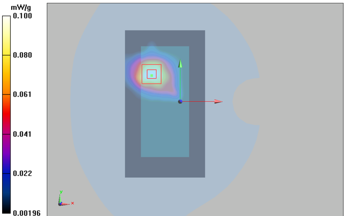
Figure 15 802.11n (HT20) Channel 11
