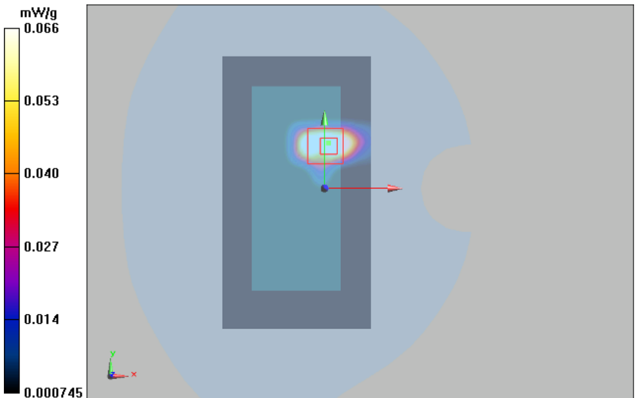
Figure 14 802.11g Chain 1 Channel 6
