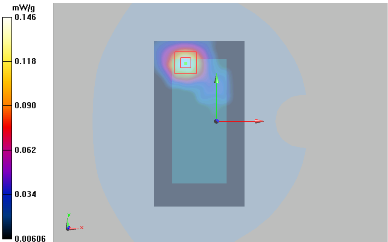
Figure 11 802.11g Chain 2 Channel 11
