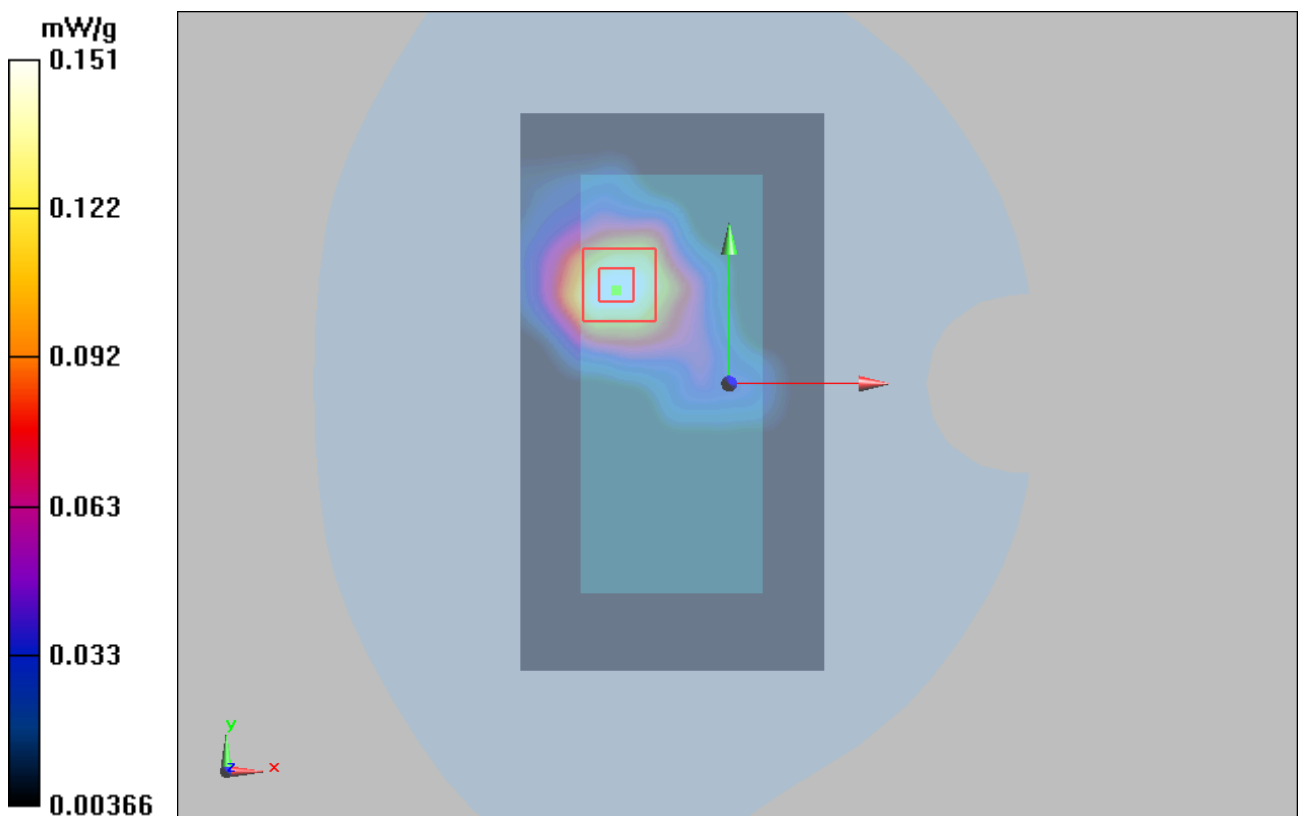
Figure 12 802.11g Chain 2 Channel 6
