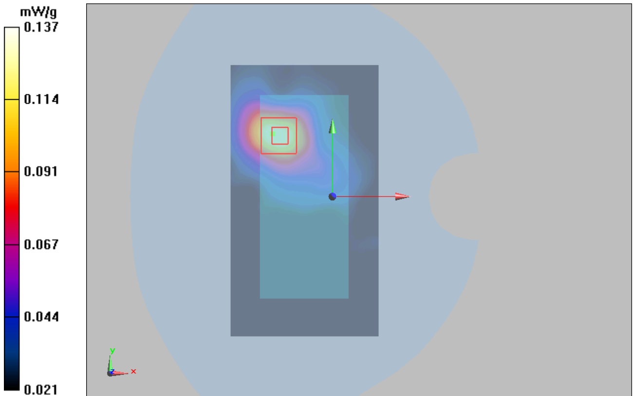
Figure 8 802.11b Chain 2 Channel 6
