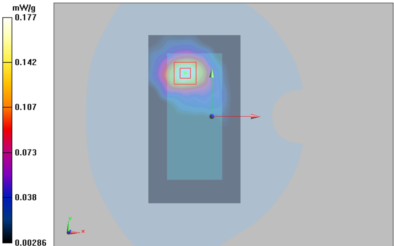
Figure 16 802.11n (HT20) Channel 6
