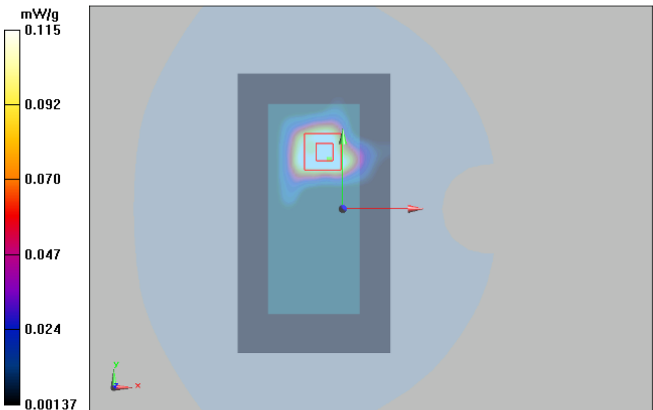
Figure 10 802.11b Chain 1 Channel 11
