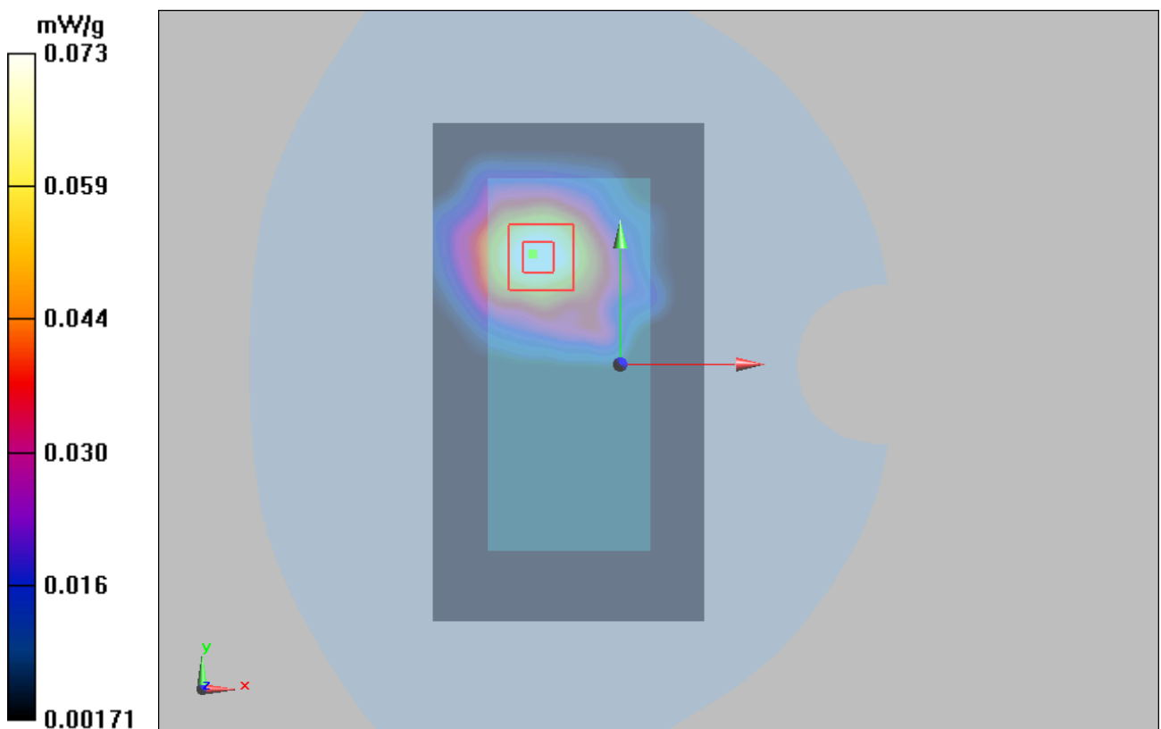
Figure 17 802.11n (HT20) Channel 1
