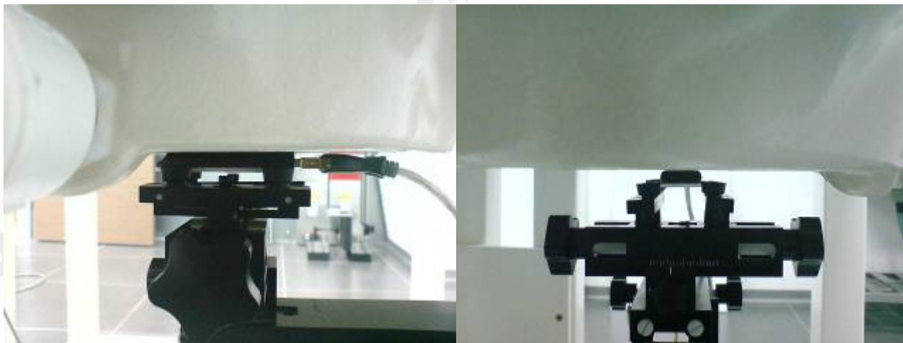
Fig 3 : Back side of the EUT is paralleled and contacted with flat phantom.
