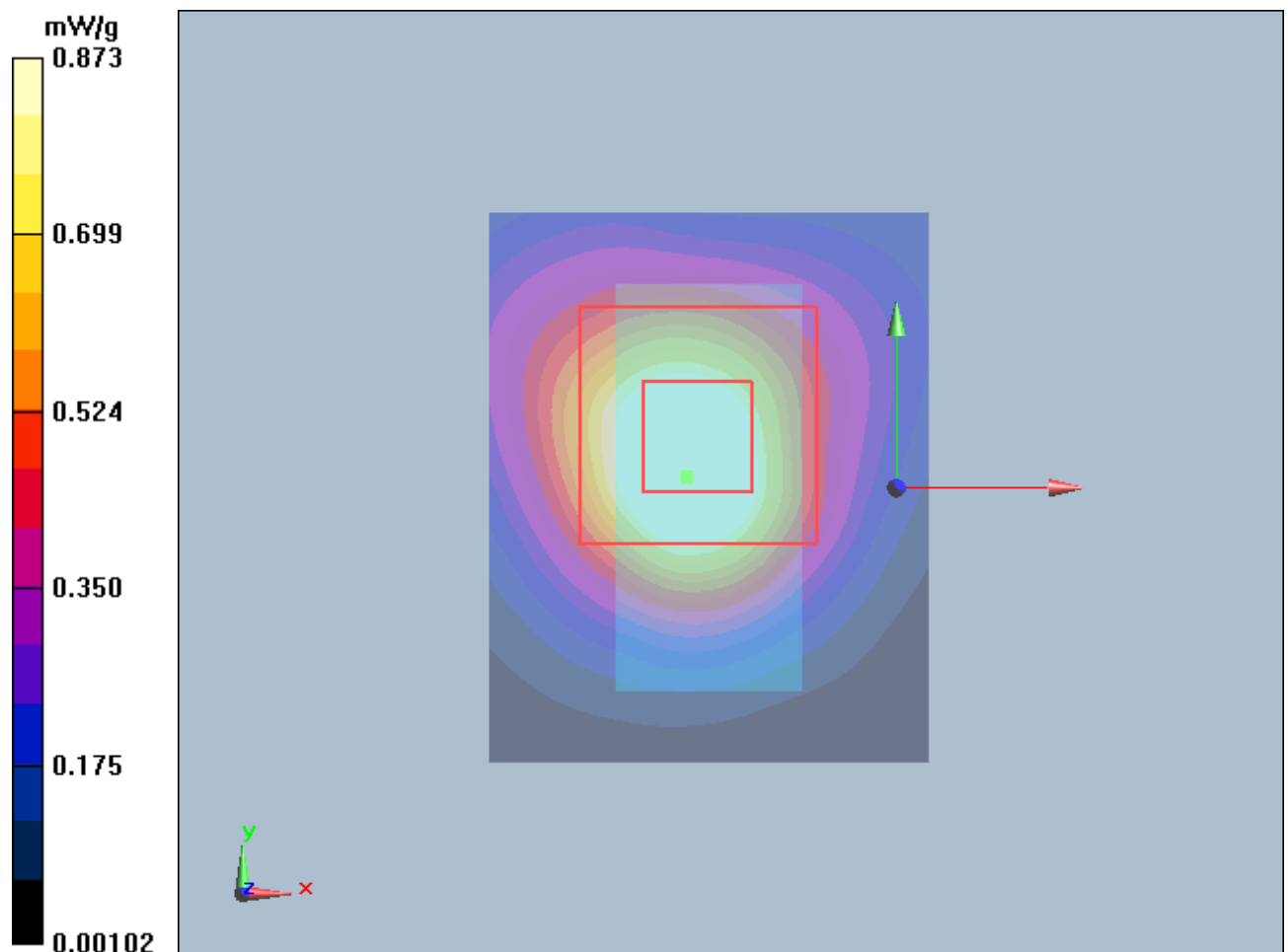
Figure 7 802.11b with IBM T61 Test Position 1 Channel 11
