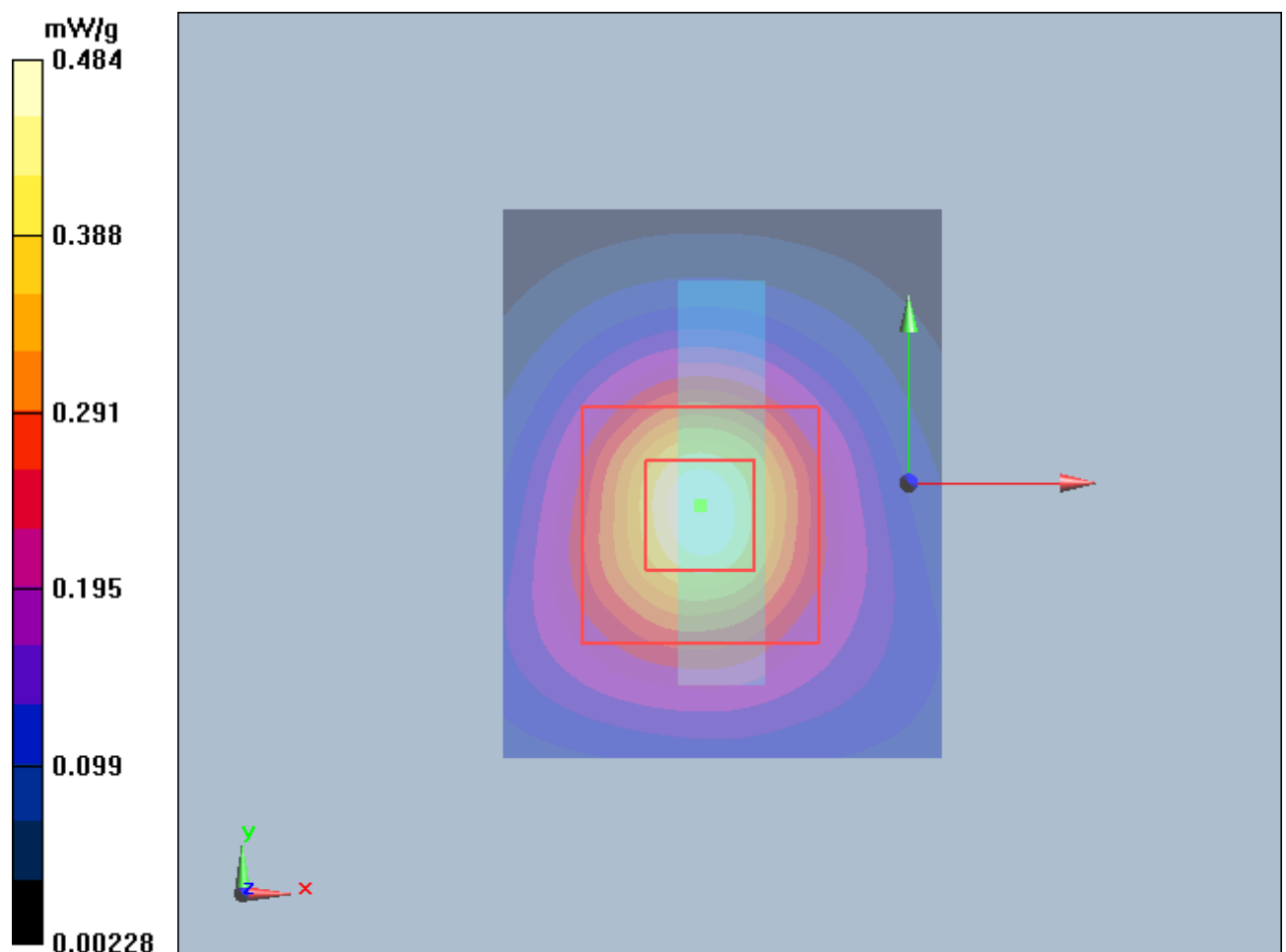
Figure 12 802.11b with IBM T61 Test Position 4 Channel 11
