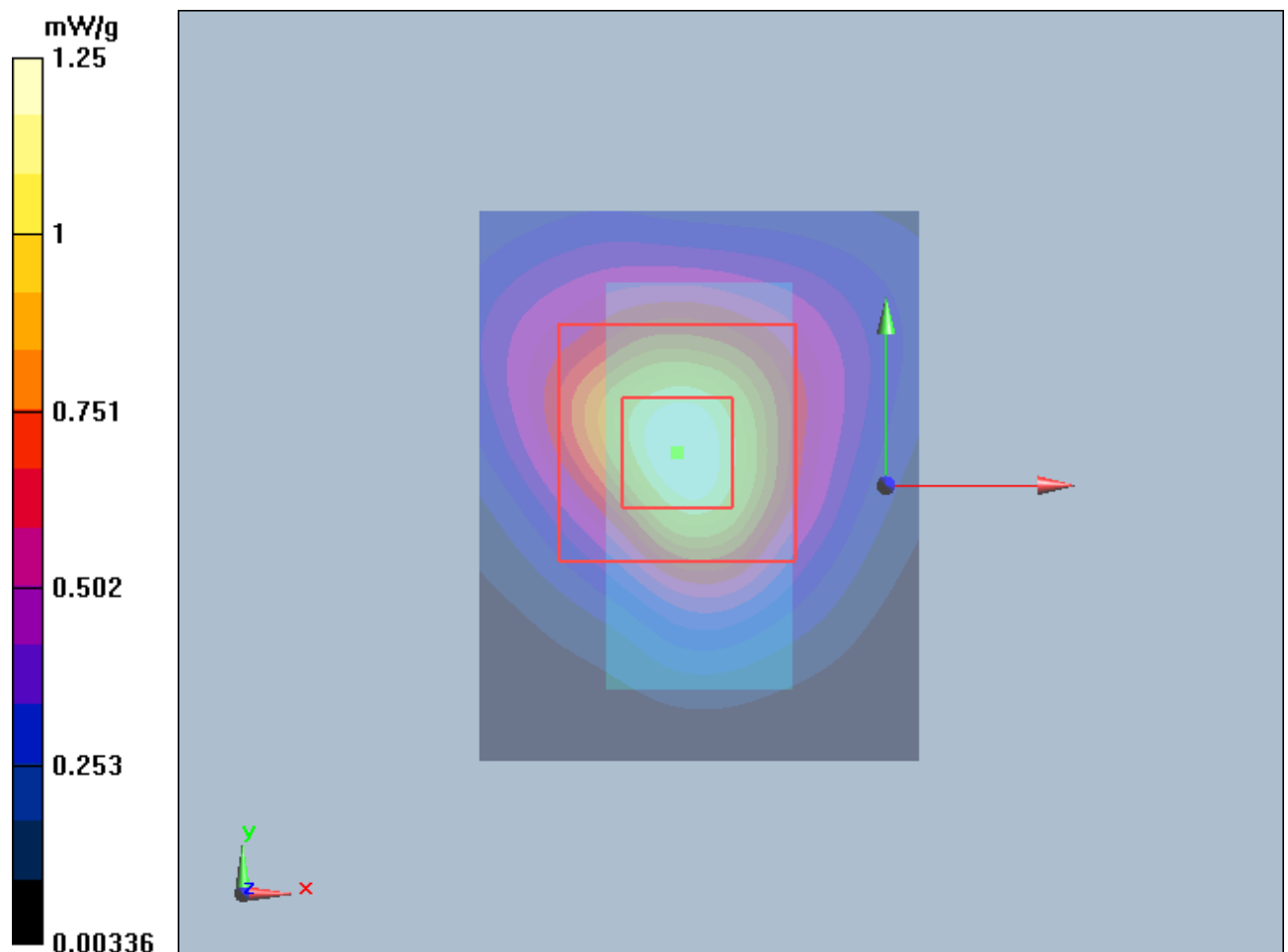
Figure 14 802.11n HT20 with IBM T61 Test Position 1 Channel 11
