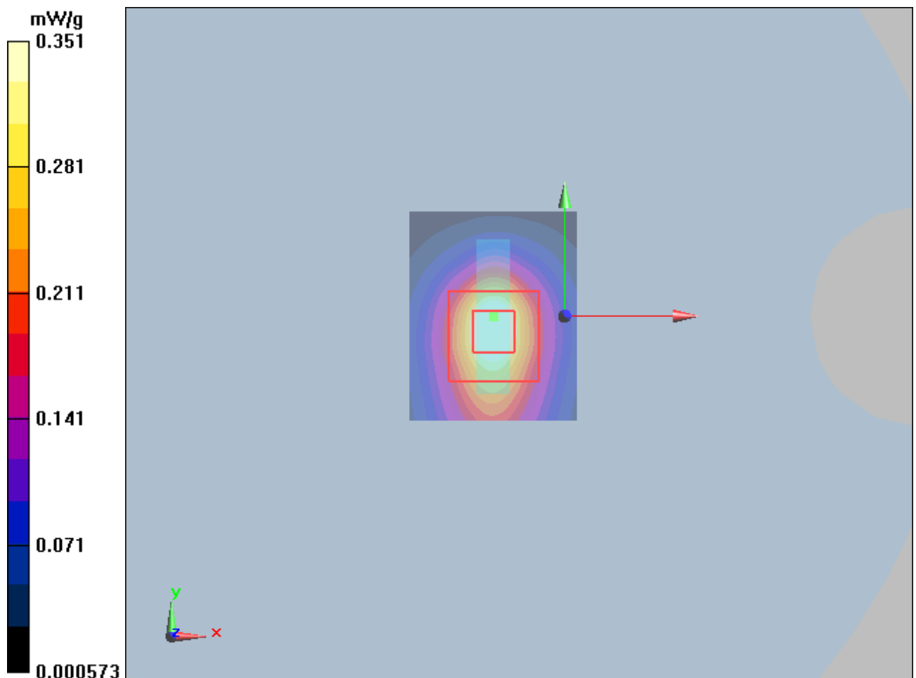
Figure 11 802.11b with IBM T61 Test Position 3 Channel 11
