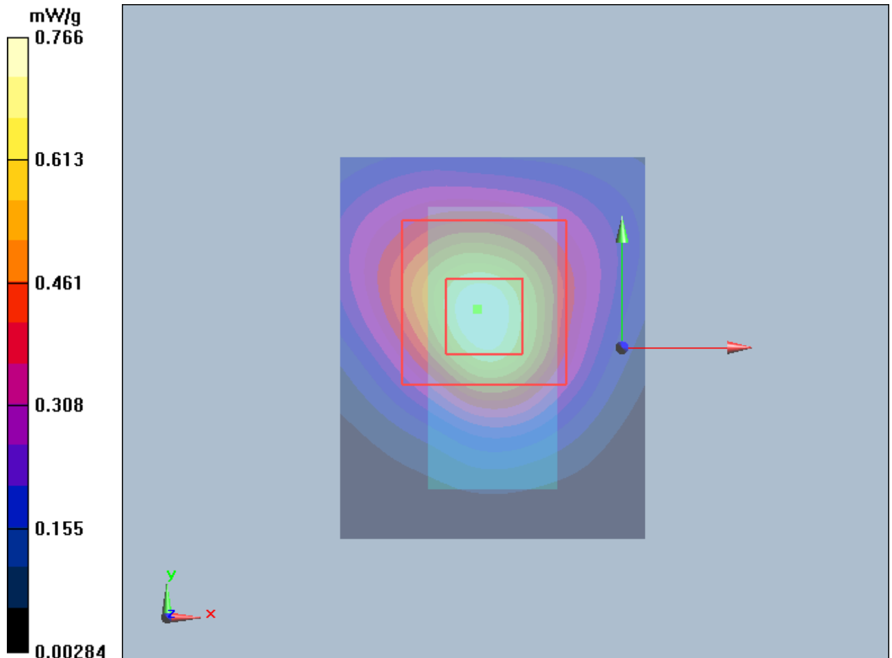
Figure 9 802.11b with IBM T61 Test Position 1 Channel 1
