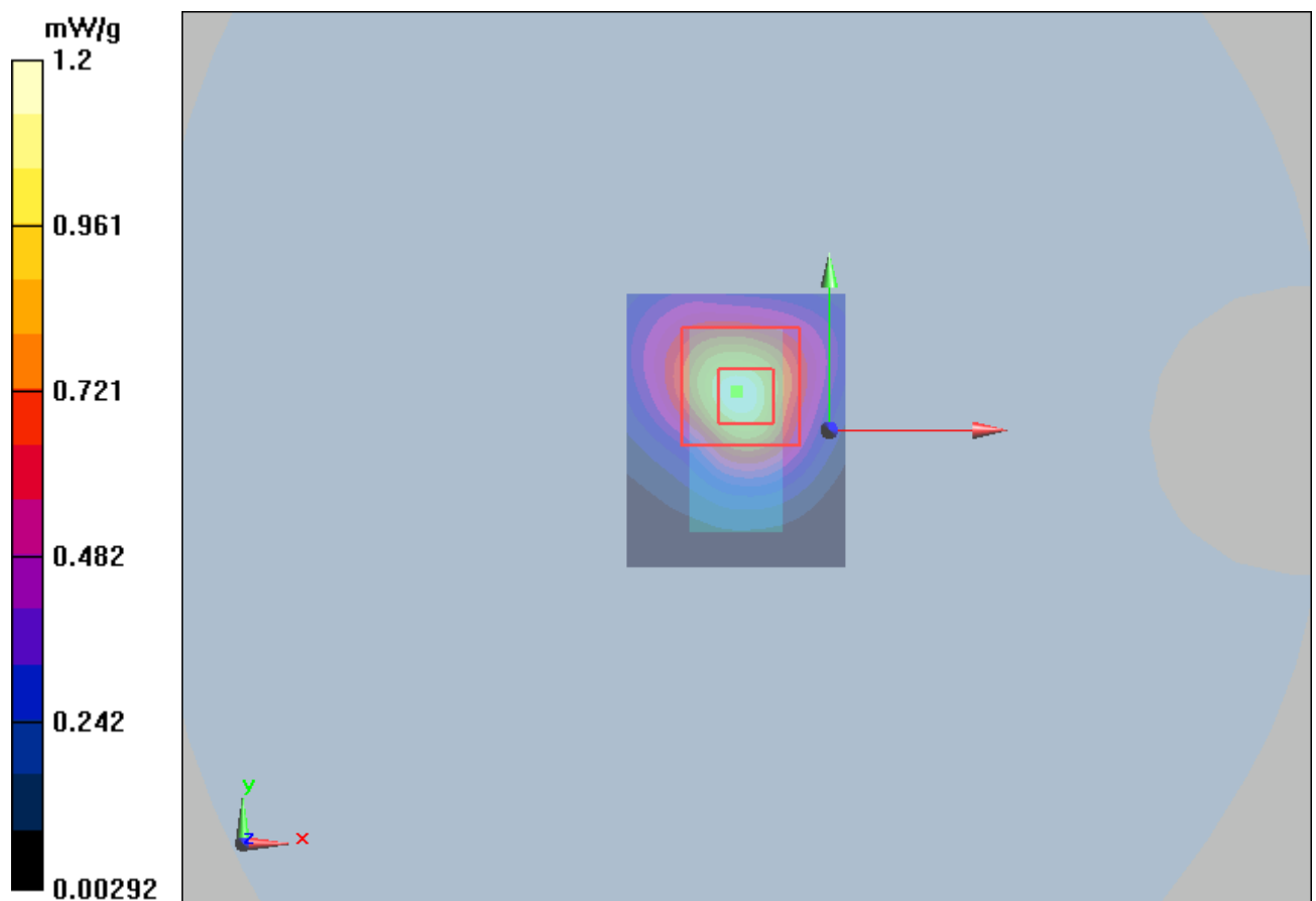
Figure 15 802.11g with IBM T61 Test Position 1 Channel 11
