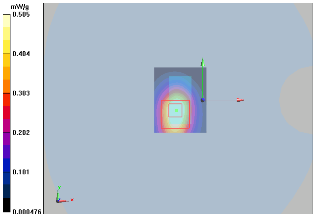
Figure 10 802.11b with IBM T61 Test Position 2 Channel 11
