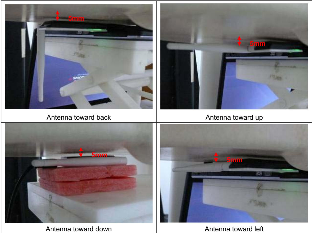
Picture 5: Test position 1
