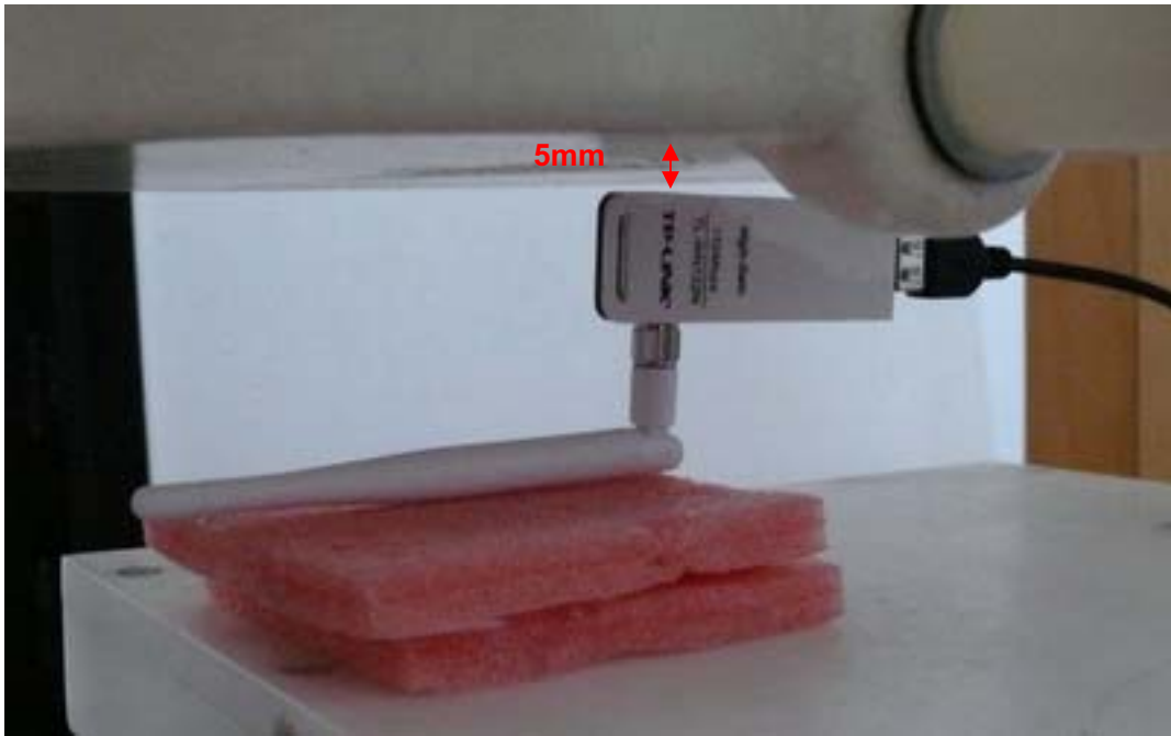
Antenna toward up Picture 7: Test position 3
