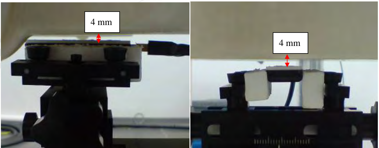
Fig.4 Front side of the EUT is paralleled with flat phantom, and spacing between EUT and Phantom is 4 mm.
