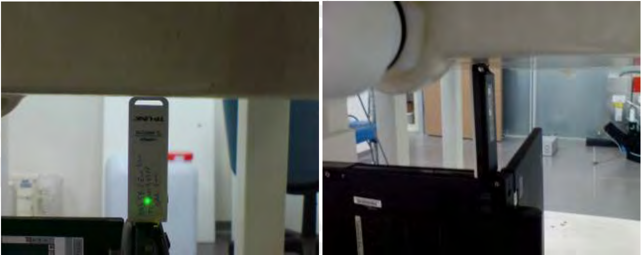
Fig.7 Tip side of EUT is paralleled with flat phantom, and contact it.
