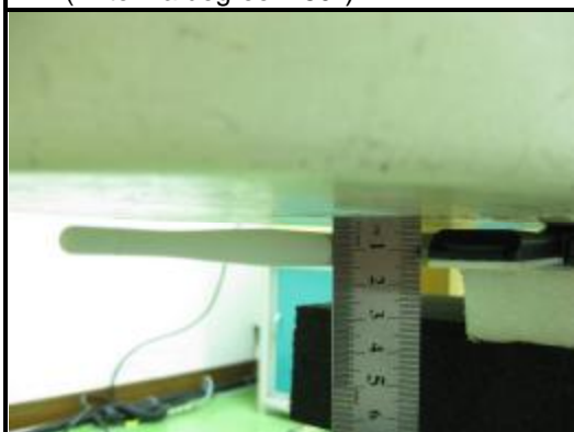
C. The bottom of the EUT face to the phantom with 5mm-separation distance. (Antenna degree: 180°)
