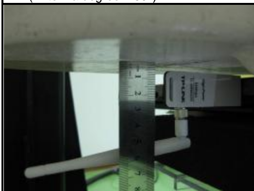
B. The right edge of the EUT face to the phantom with 5mm-separation distance. (Antenna degree: 180°)
