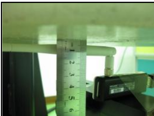
A. The left edge of the EUT face to the phantom with 5mm-separation distance. (Antenna degree: 180°)
