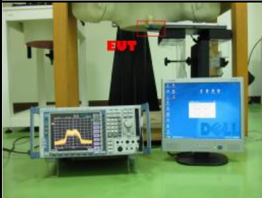
Test Setup Photo
