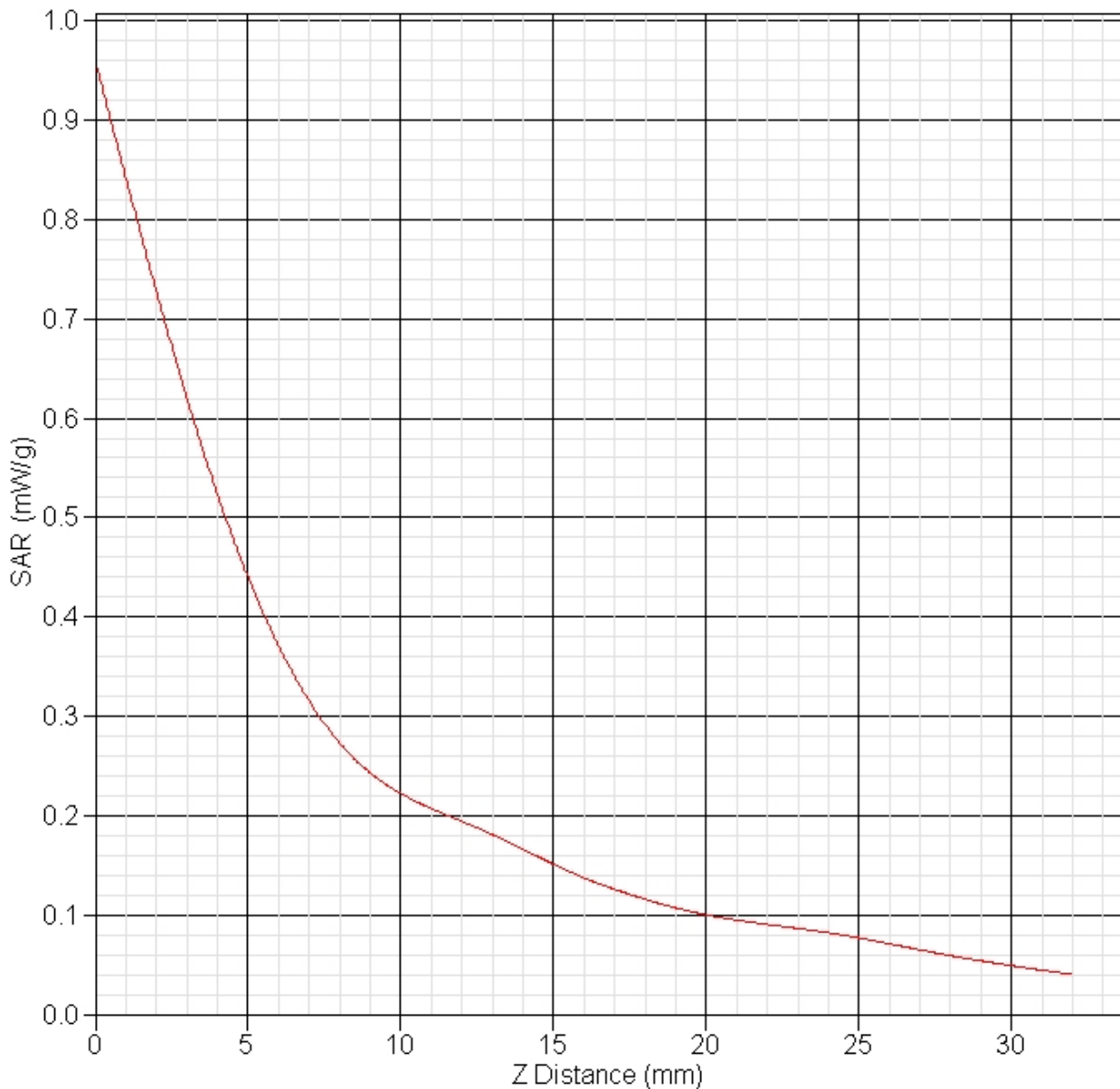
SAR-Z Axis at Hotspot x:0.06 y:-2.01
