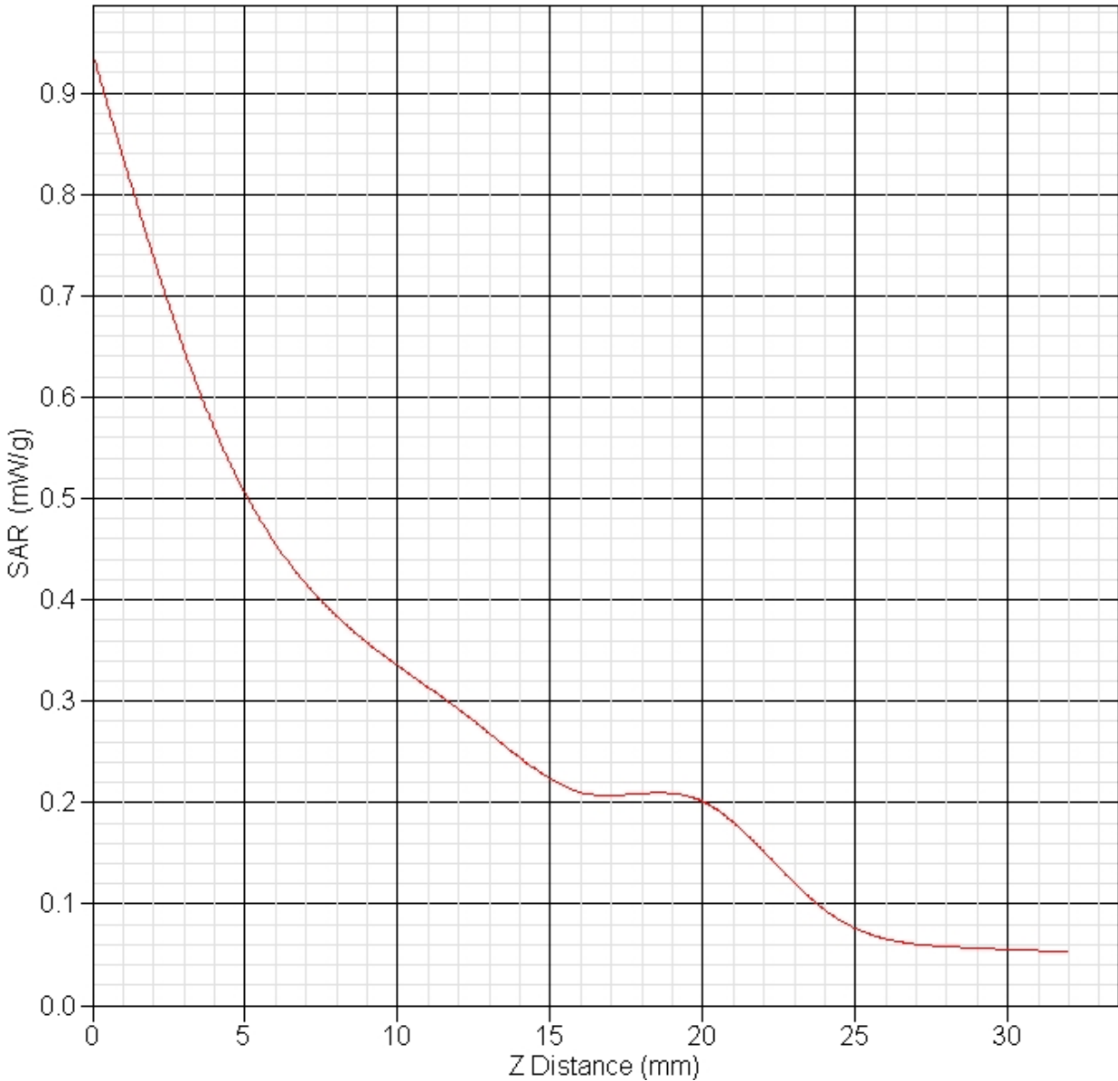
SAR-Z Axis at Hotspot x:0.06 y:-6.01
