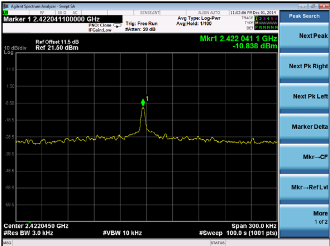
Test Mode: IEEE 802.11n HT40 TX Test CH3: 2422MHz
