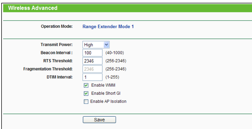
Figure 4-22 Wireless Advanced
