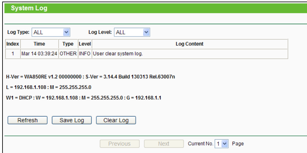
Figure 4-35 System Log
