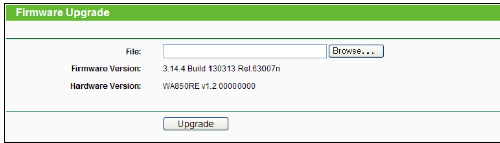
Figure 4-30 Firmware Upgrade
