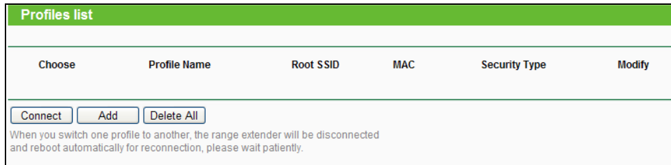
Figure 4-11 Profile
