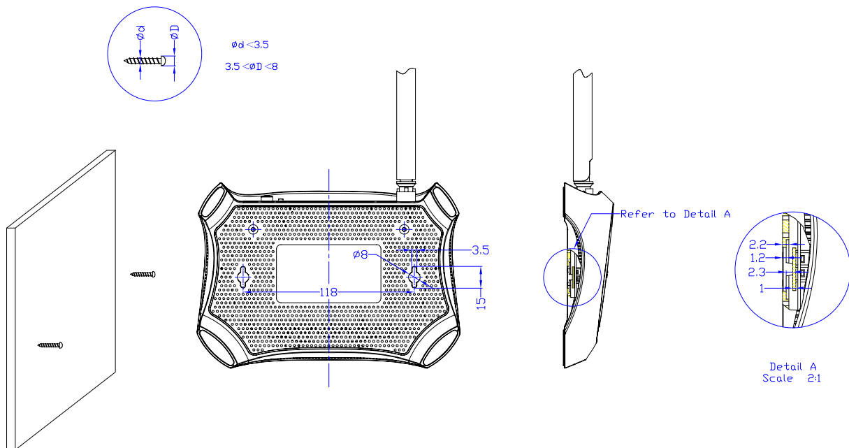
Figure 2-3 Wall-mount Install
