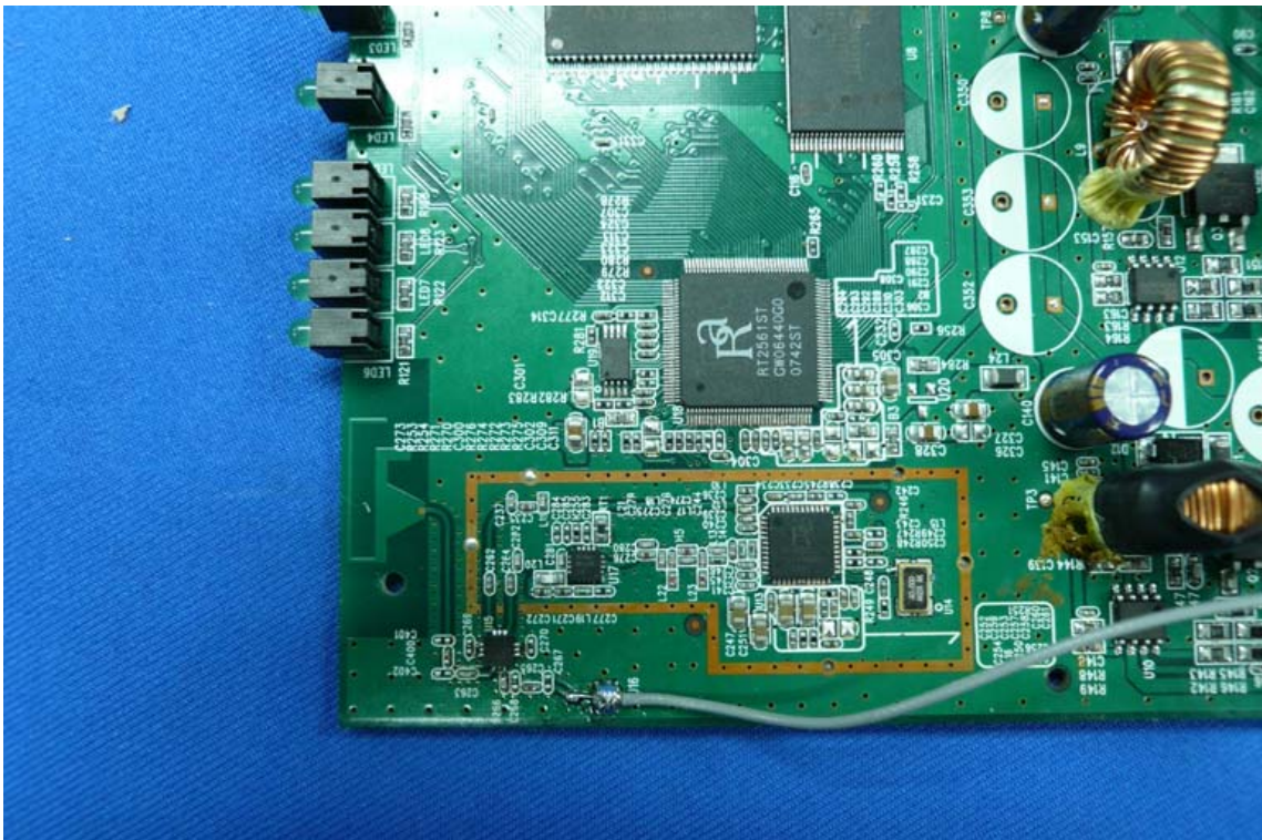
Figure 10 Inside of the EUT
