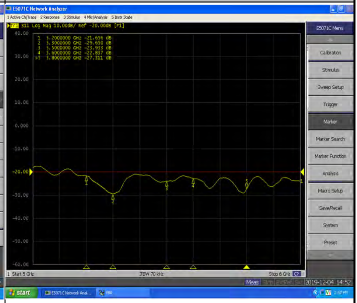
Return Loss-Head
