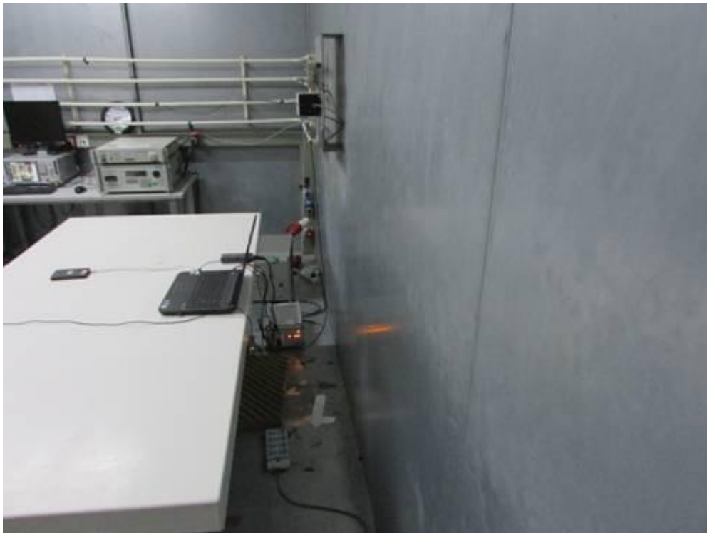
Test Mode: TransmitDescription: Back View of Conducted Emission Test Setup
