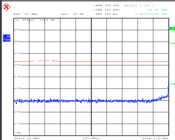
Spurious Emission 30MHz~2.4GHz
