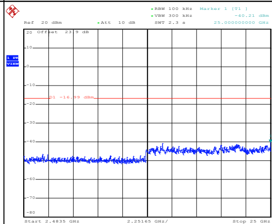
Spurious Emission 2.4835GHz~25GHz
