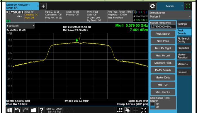
Channel 116 (5580MHz)
