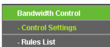
Figure 5-65 Bandwidth Control
