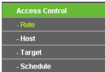
Figure 4-51 Access Control
