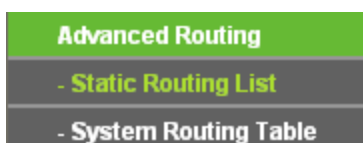
Figure 4-66 Advanced Routing
