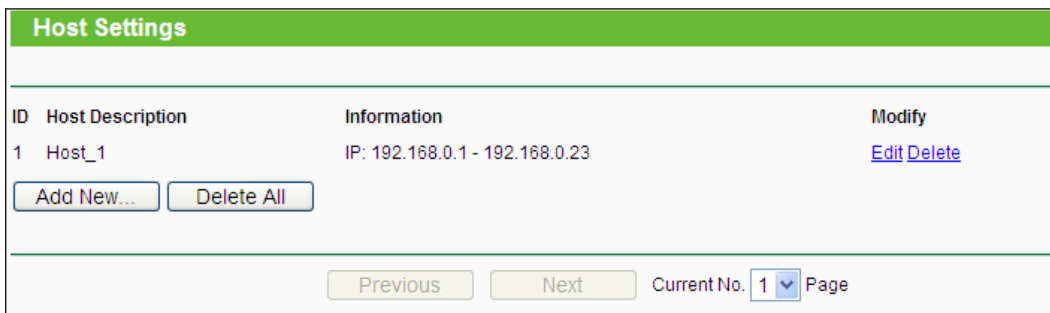
Figure 4-58 Host Settings
