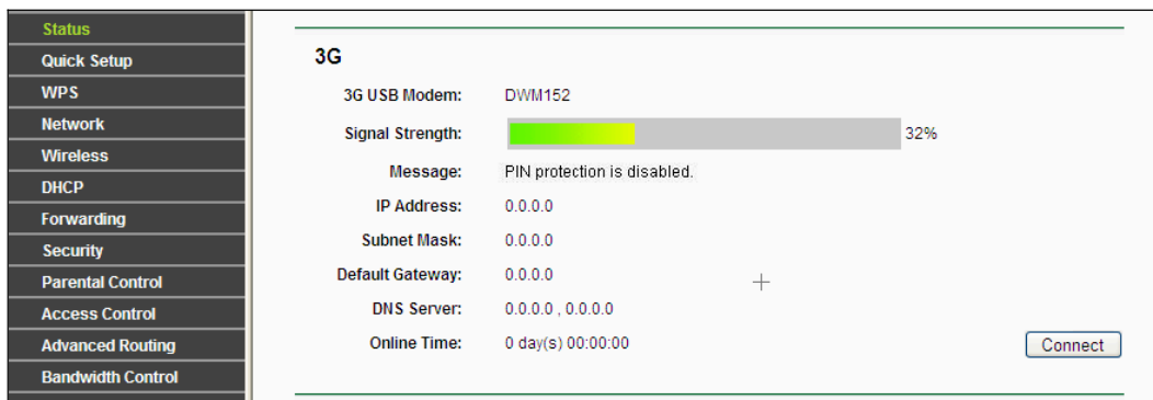
Figure 3-3 Status – 3G
