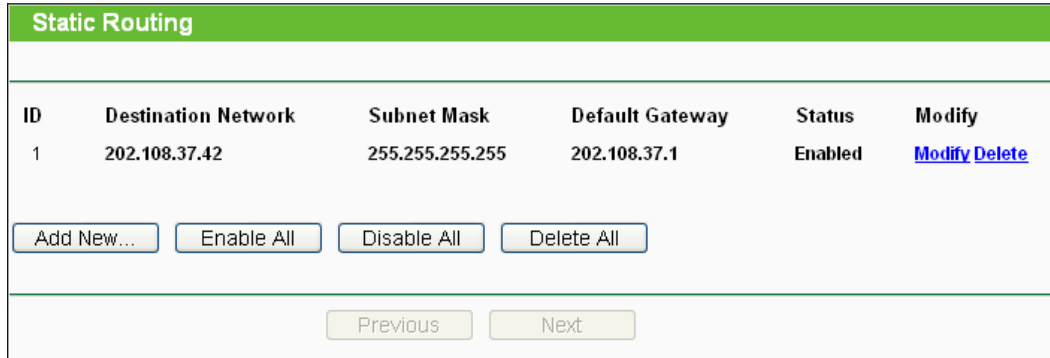
Figure 4-67 Static Routing
