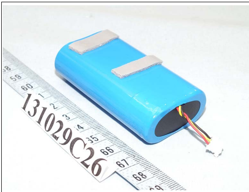
Battery 1 (Brand: HUIZHOU DESAY BATTERY CO.,LTD / Model: TBL-18B5200)
