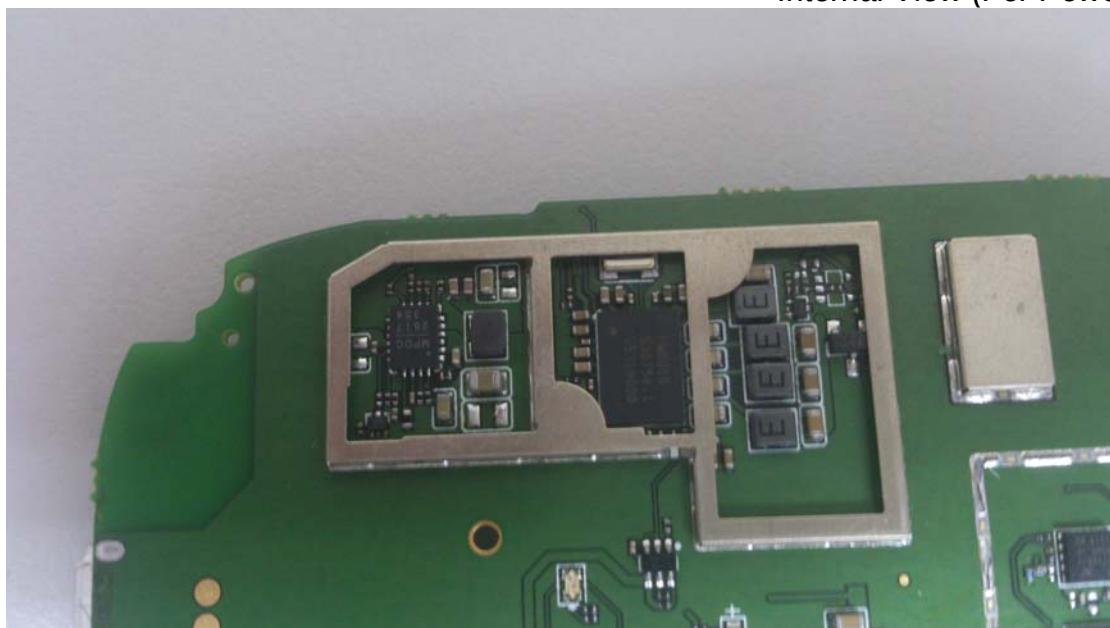
Photo 9 Internal View (WiFi Module)
