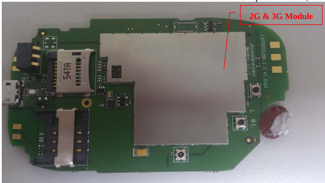
Photo 7 Internal View (Main Board, Back View)
