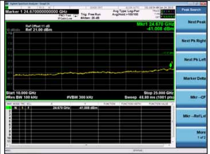
Test CH4: 2437MHz(10GHz – 25GHz)
