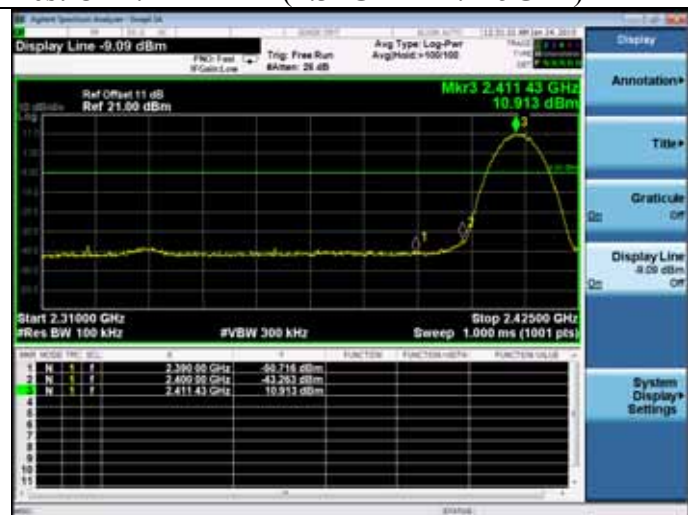
Test CH1: 2412MHz(2.31GHz – 2.425GHz)
