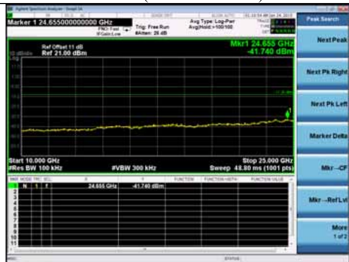
Test CH4: 2437MHz(10GHz – 25GHz)
