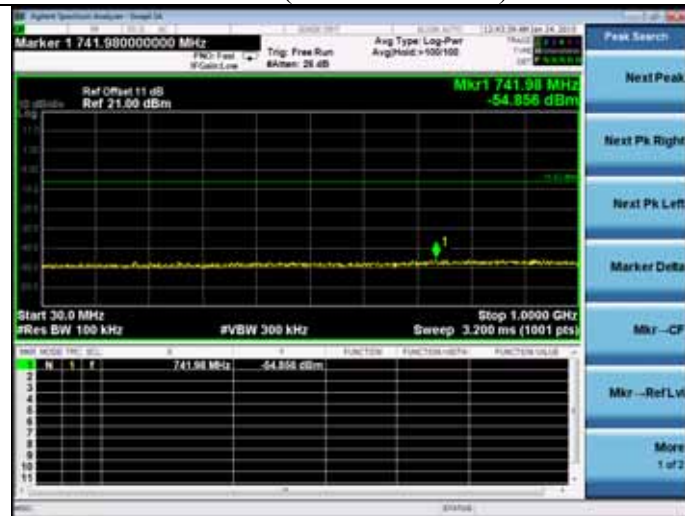
Test CH1: 2412MHz(30MHz – 1GHz)
