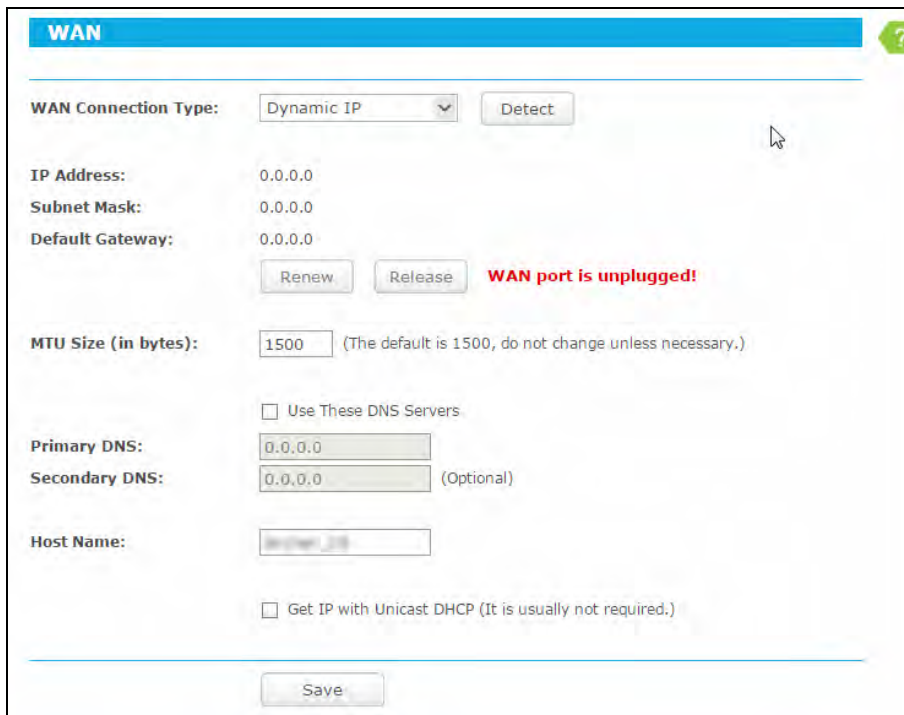
Figure 5-3 WAN – Dynamic IP
