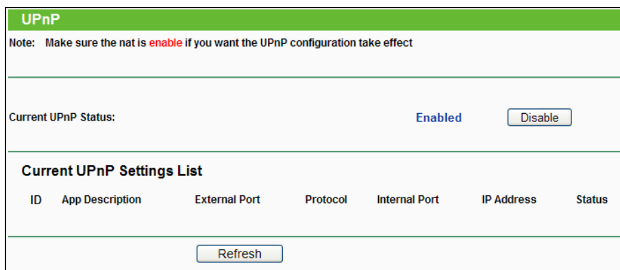
Figure 4-64 UPnP Setting
