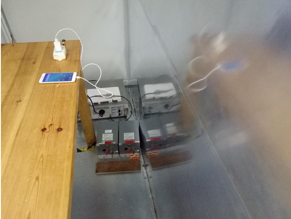
Conducted Emission Test BT
