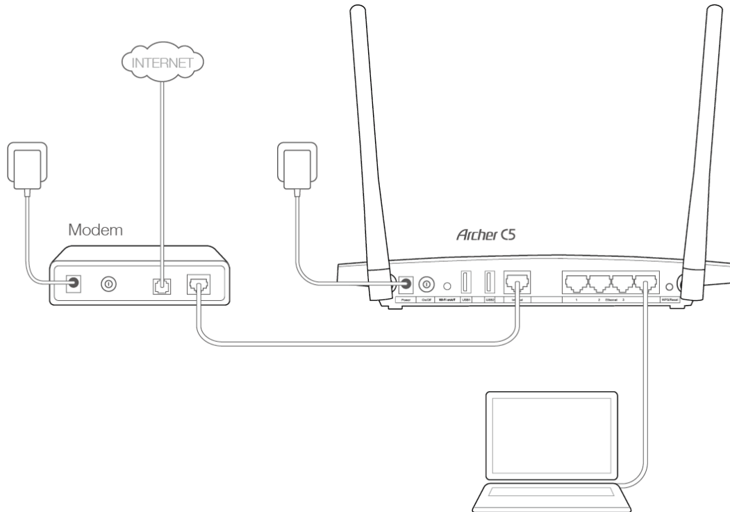
Figure 2-1 Hardware Installation
