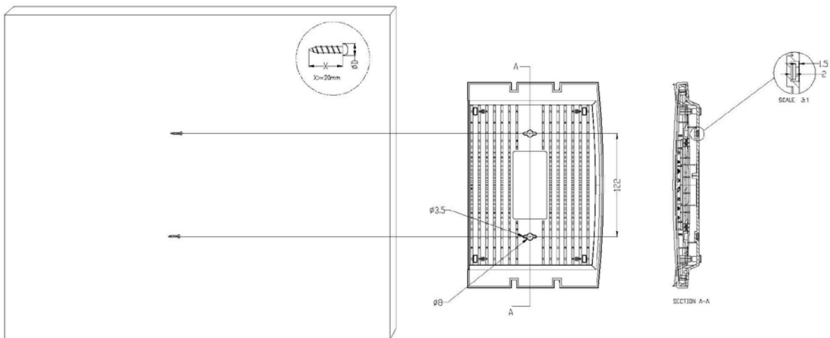
Figure 2-2 Wall-mount Installation
