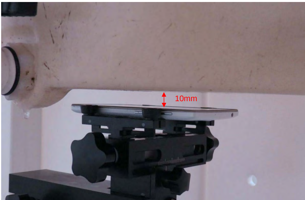
Picture 19: Front Side, the distance from handset to the bottom of the Phantom is 10mm
