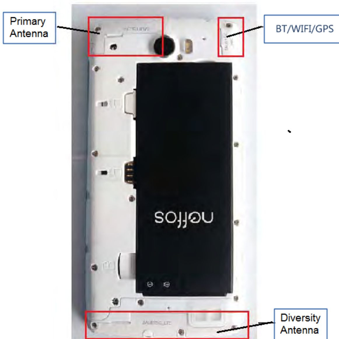
c: Antenna
