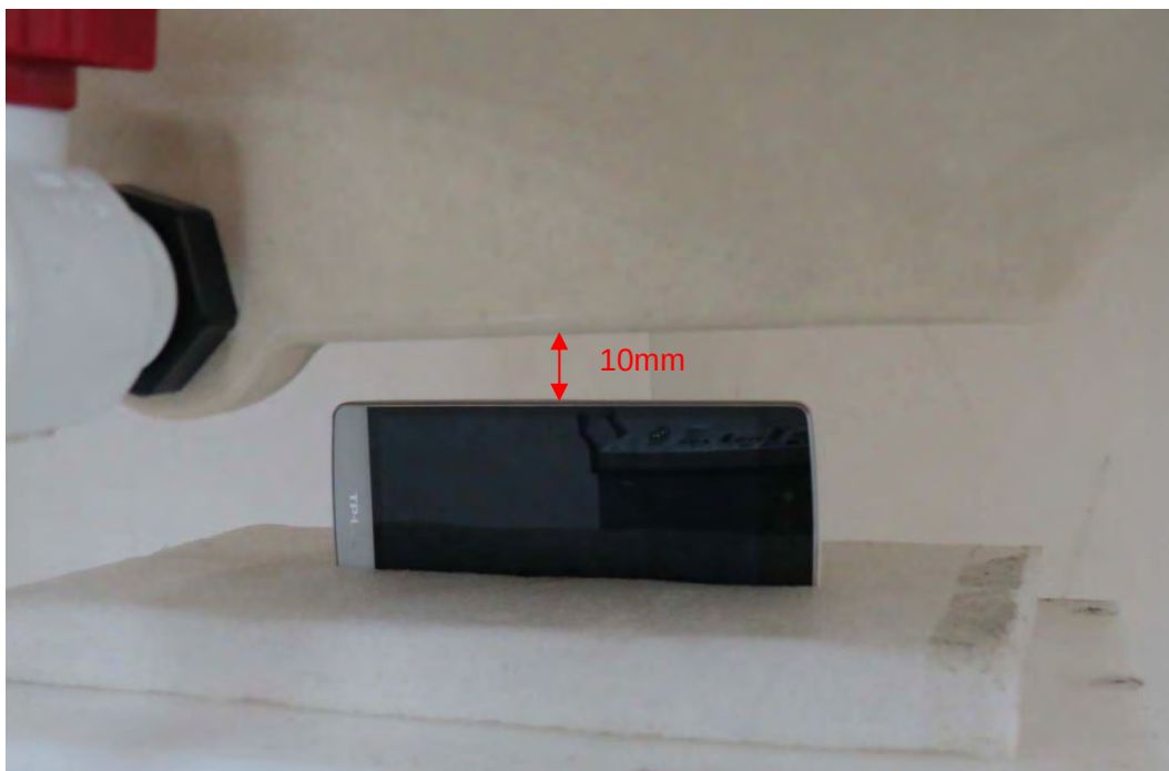
Picture 20: Left Side, the distance from handset to the bottom of the Phantom is 10mm
