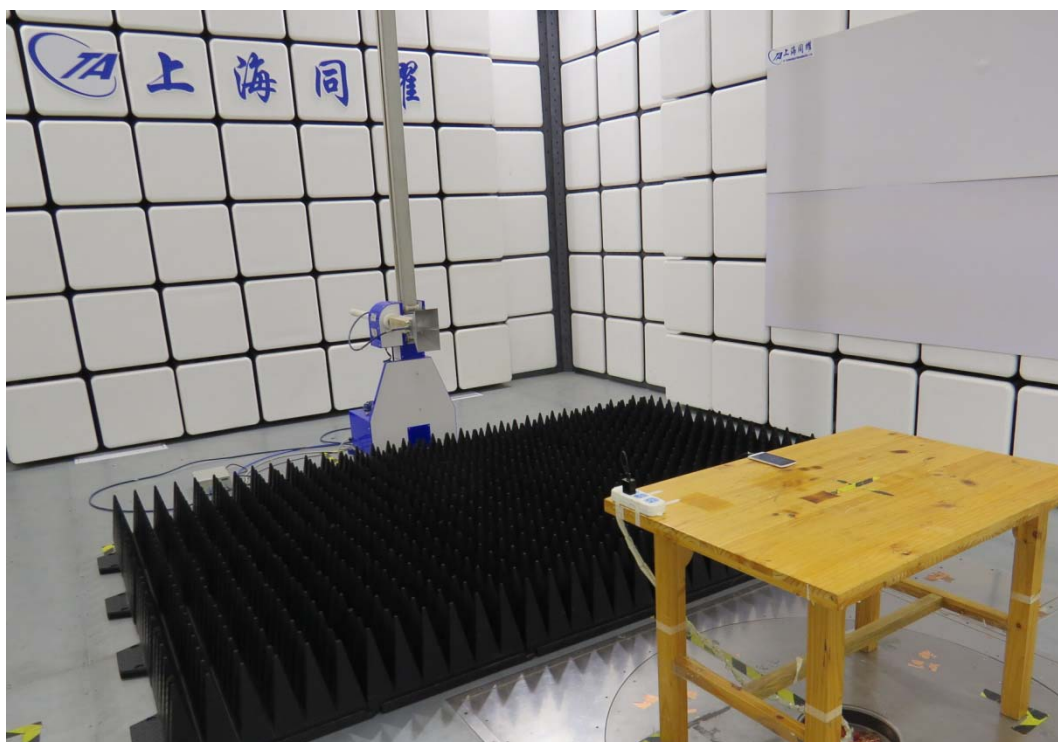
Above 1GHz Radiated Emission Test Setup
