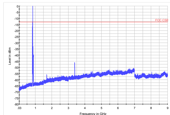
WCDMA Band V CH4233 30MHz~9GHz
