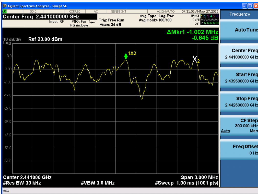
3DH5 Carrier frequency (MHz): 2441
