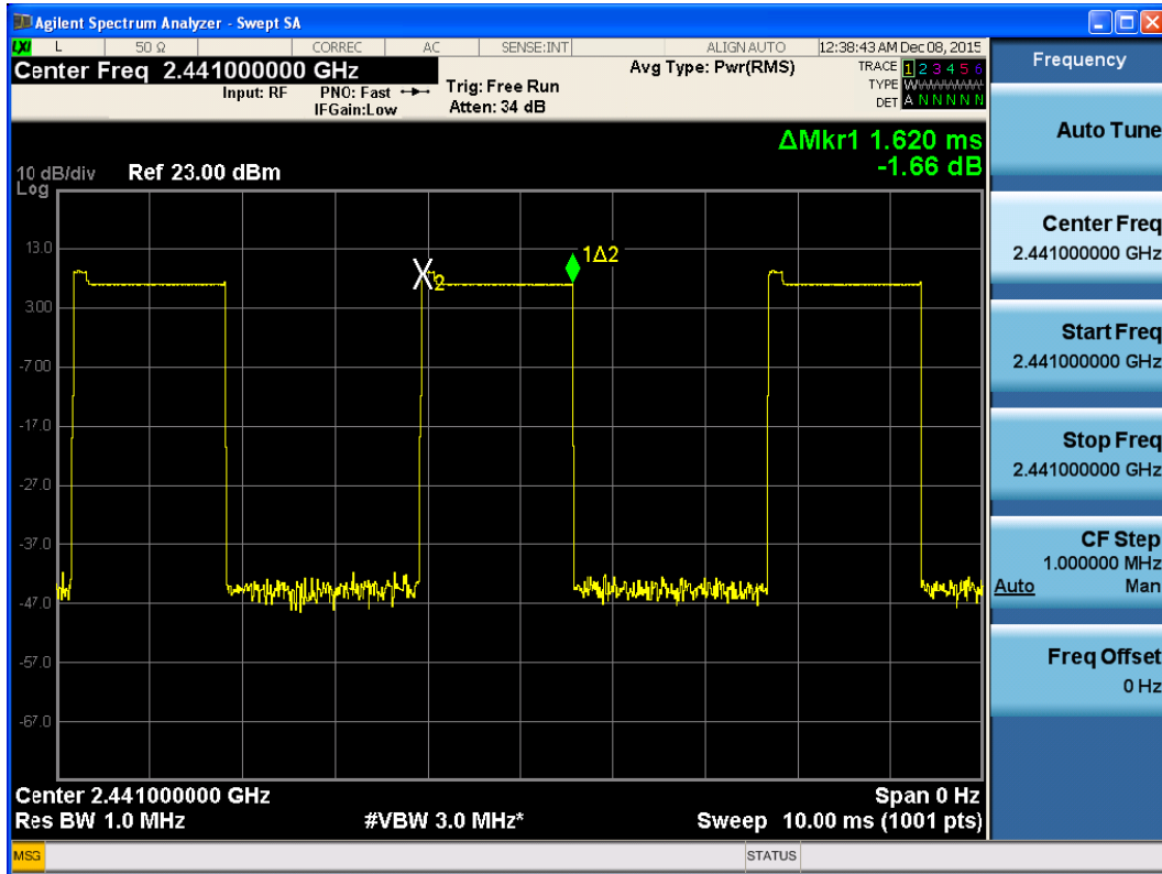
Carrier frequency (MHz): 2441, 3DH3
