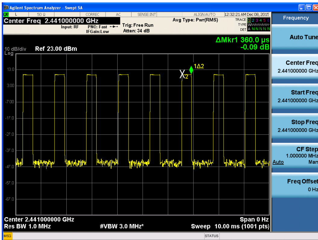
Carrier frequency (MHz): 2441, DH1
