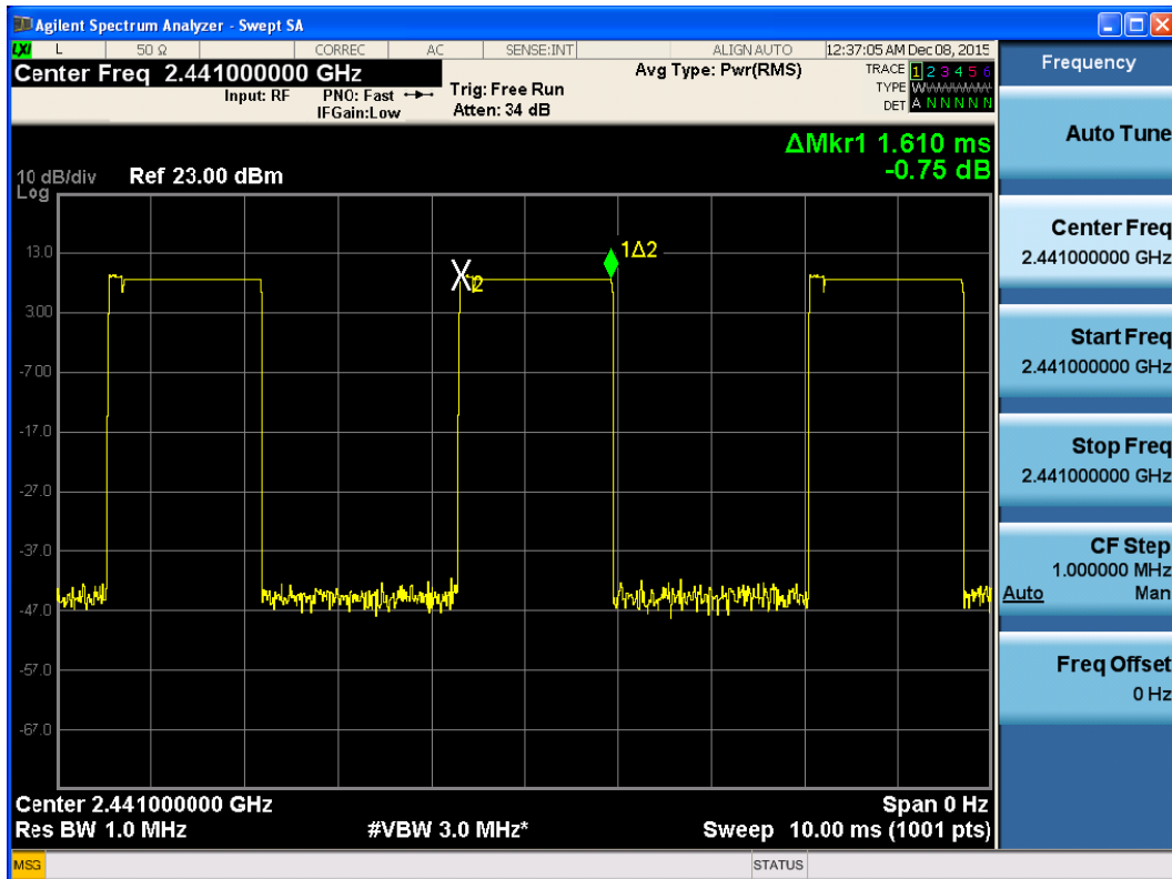
Carrier frequency (MHz): 2441, 2DH3
