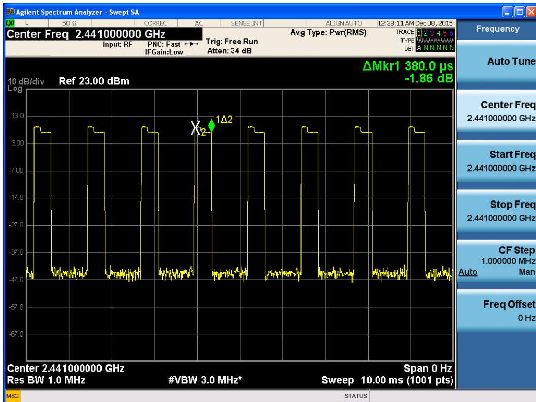
Carrier frequency (MHz): 2441, 3DH1
