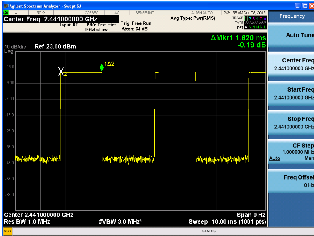
Carrier frequency (MHz): 2441, DH3
