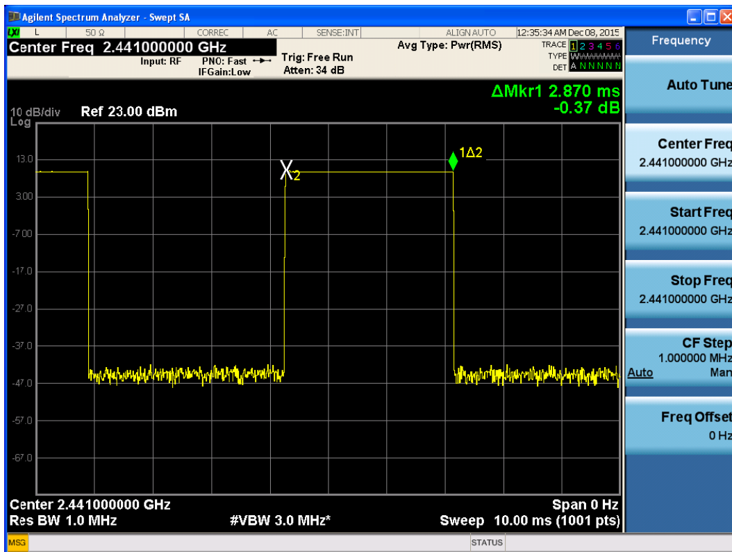
Carrier frequency (MHz): 2441, DH5
