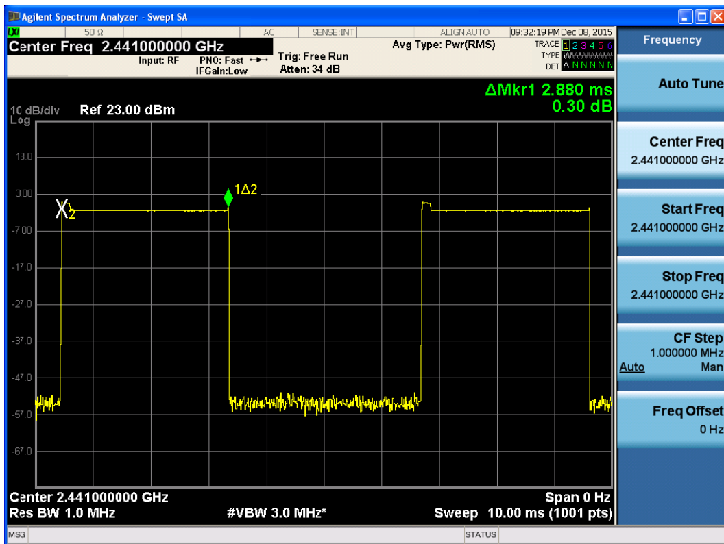
Carrier frequency (MHz): 2441, 3DH5
