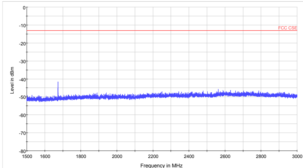
Spurious conducted emissions from 1.5GHz~3GHz
