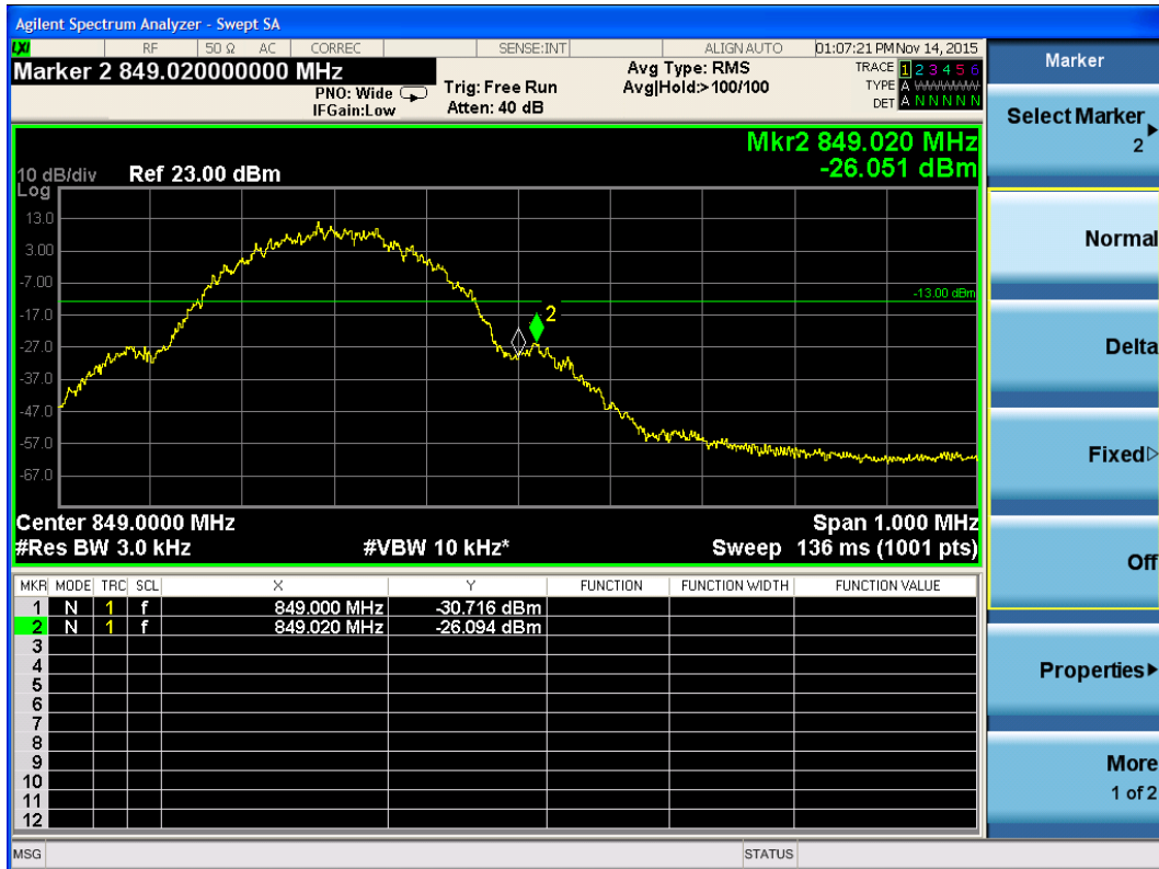
GSM 850 Channel 251
