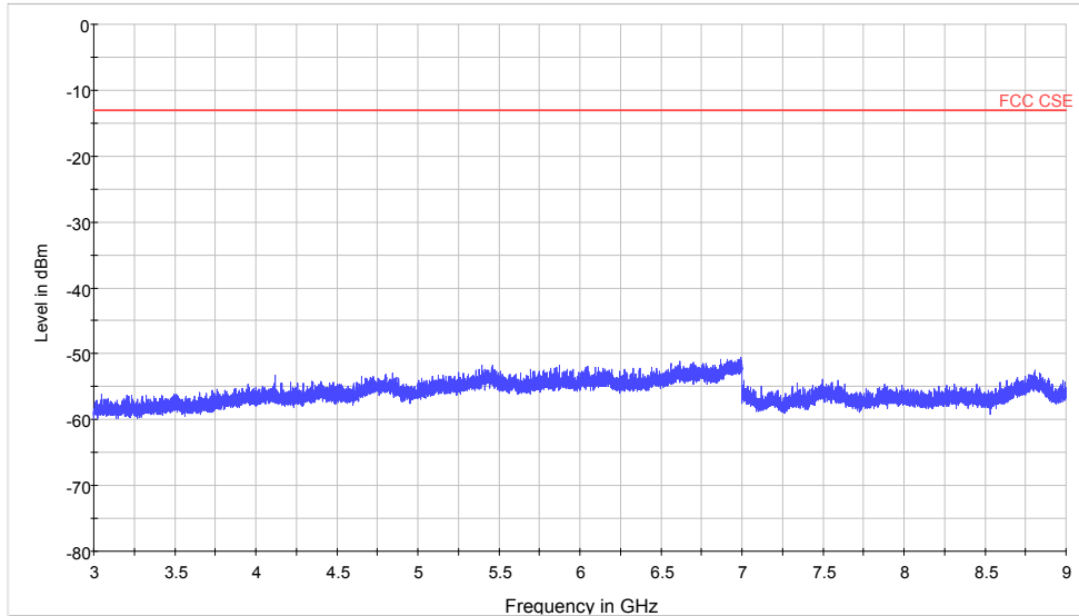
Spurious conducted emissions from 3GHz~9GHz
