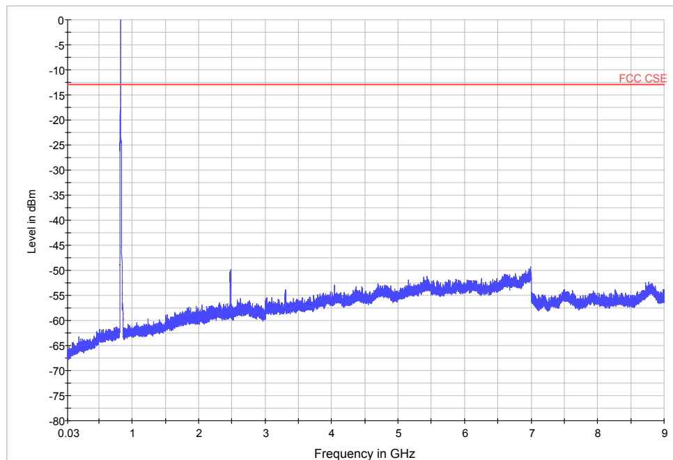
Note: The signal beyond the limit is carrier Spurious conducted emissions from 30MHz~9GHz
