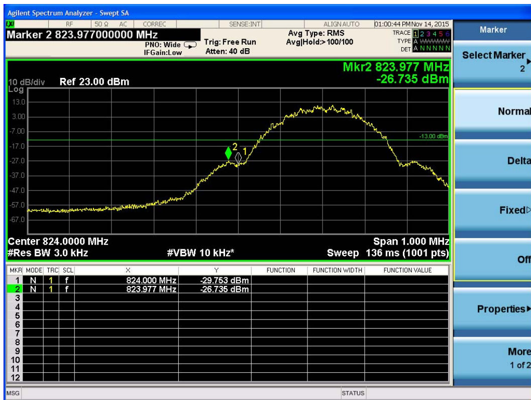
GSM 850 Channel 128
