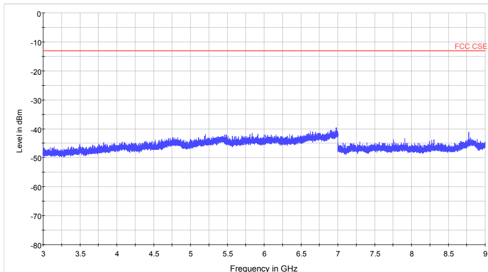
Note: The signal beyond the limit is carrier Spurious conducted emissions from 3GHz~9GHz
