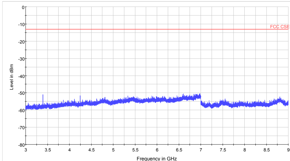
Spurious conducted emissions from 3GHz~9GHz
