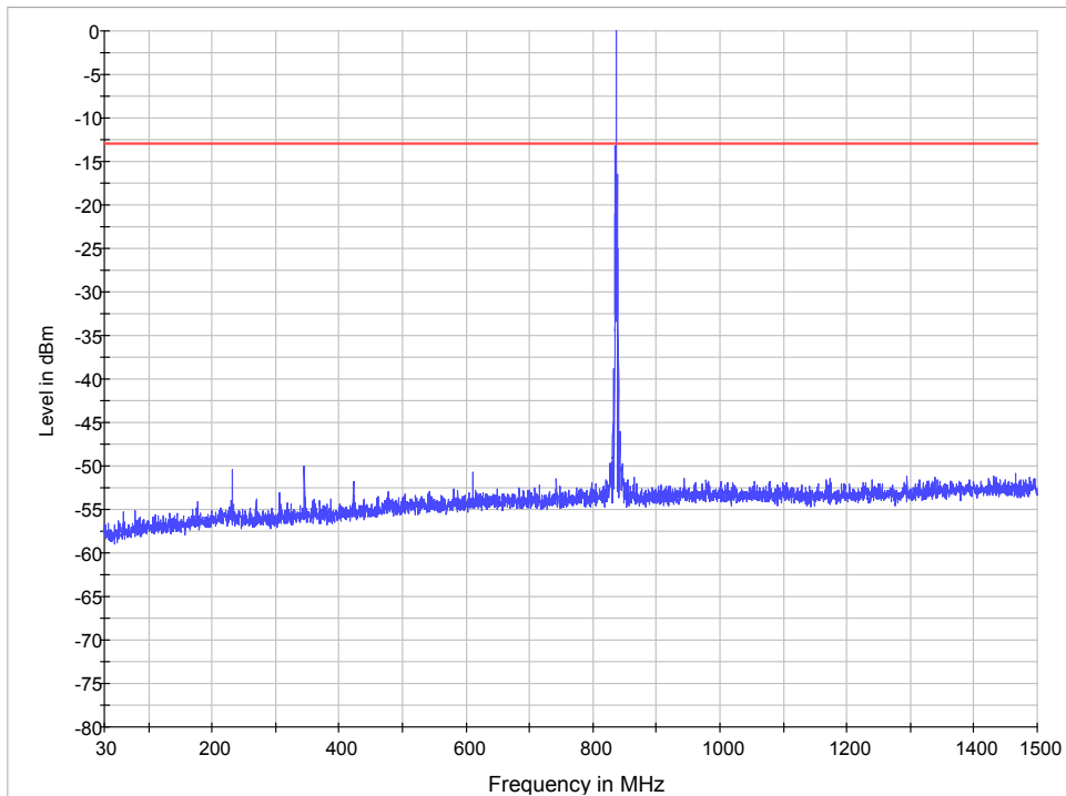
Note: The signal beyond the limit is carrier Spurious conducted emissions from 30MHz~1.5GHz
