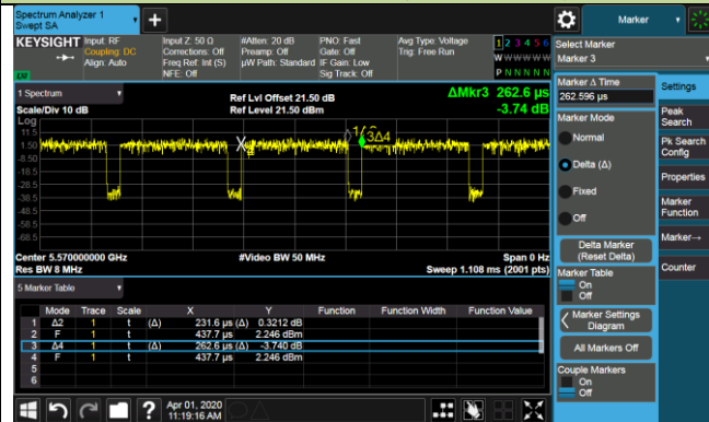
802.11ax-HE160 (T=231.6us)
