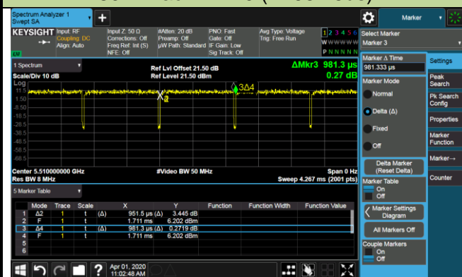
802.11ac-VHT40 (T=951.5us)
