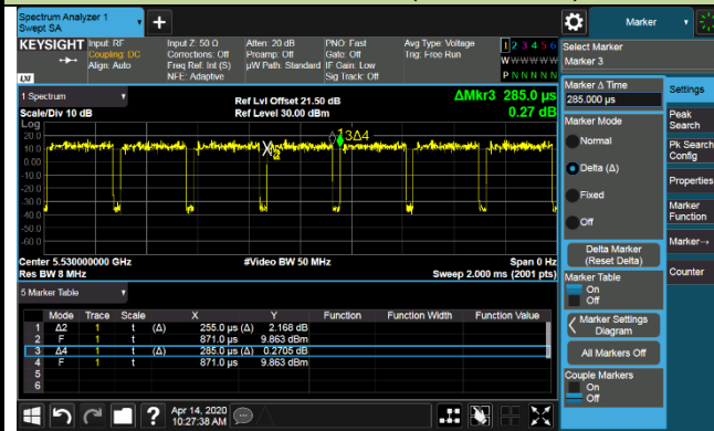
802.11ax-HE20 (T=777.7us)
