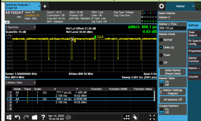
802.11ax-HE20 (T=777.7us)
