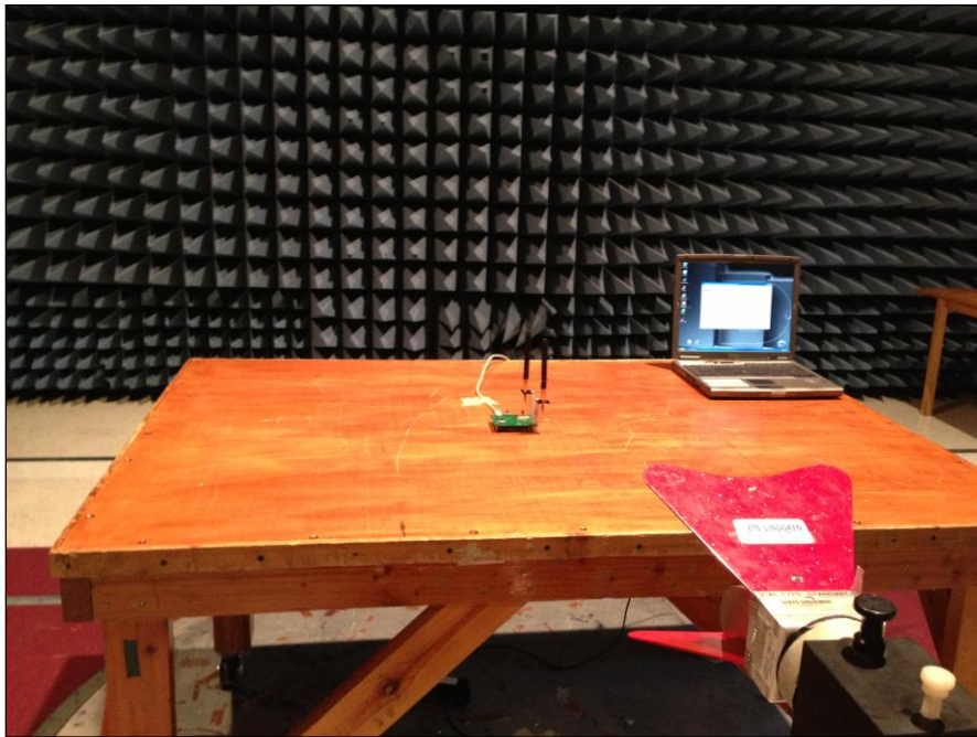
Photograph 8. Radiated Spurious Emissions, Test Setup, 1 m
