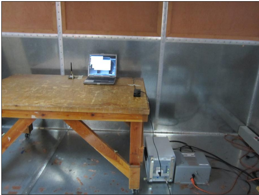
Photograph 6. Conducted Emissions, 15.207(a), Test Setup
