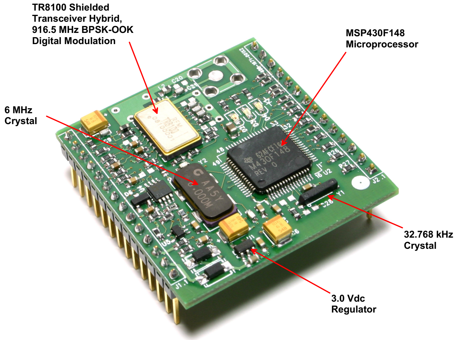
DM2200 Module FCC Reference Photo #2
