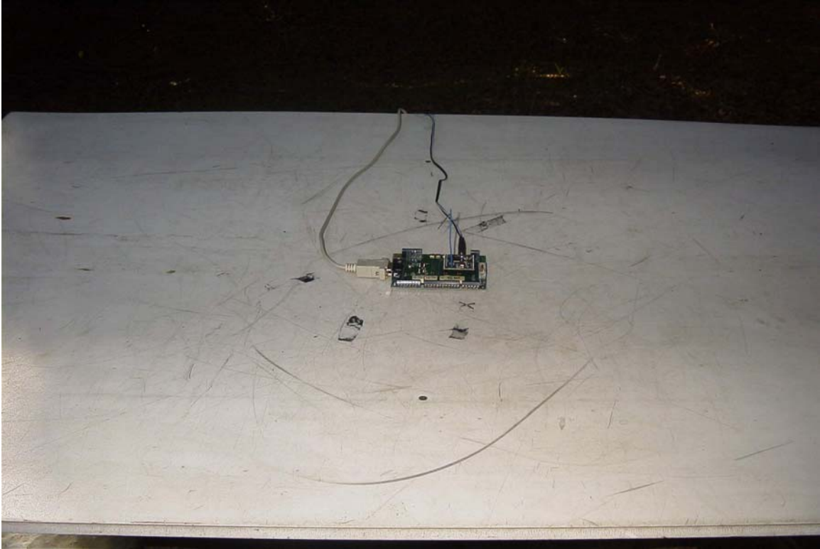
RADIATED EMISSIONS TEST SET UP WITH ¼ WAVE ANTENNA, RFM PART NO. 400-1595-001
