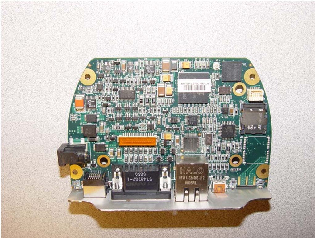
Integral Antenna PCB Assembly Top
