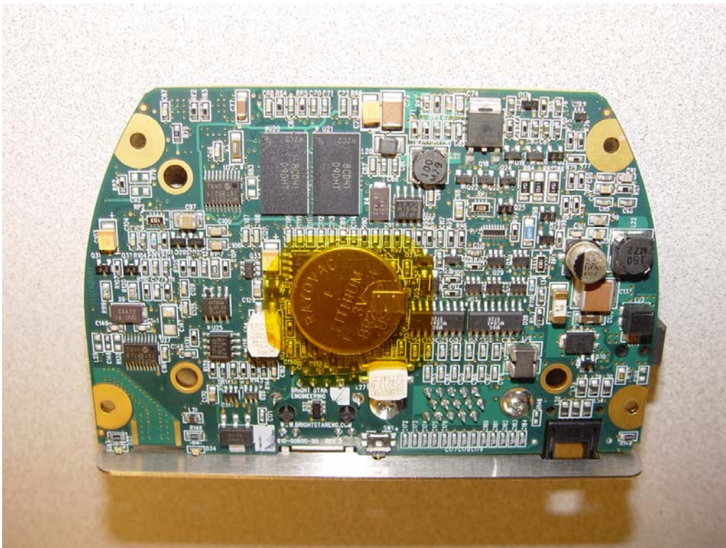
External Antenna PCB Assembly Bottom
