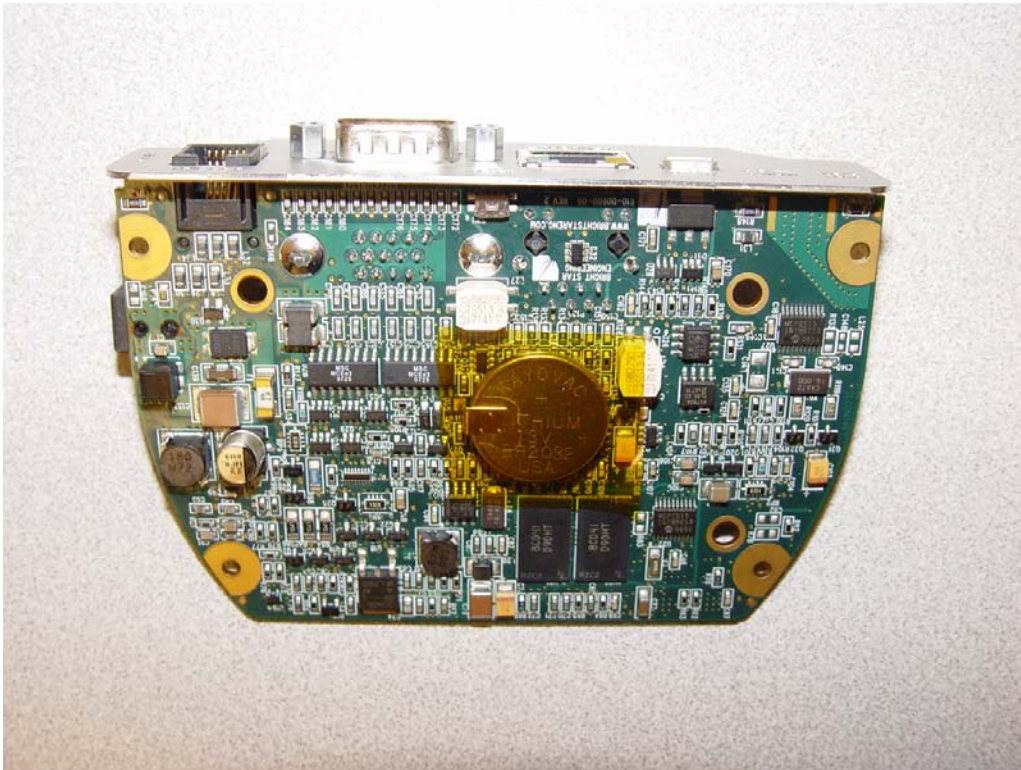
Integral Antenna PCB Assembly Bottom
