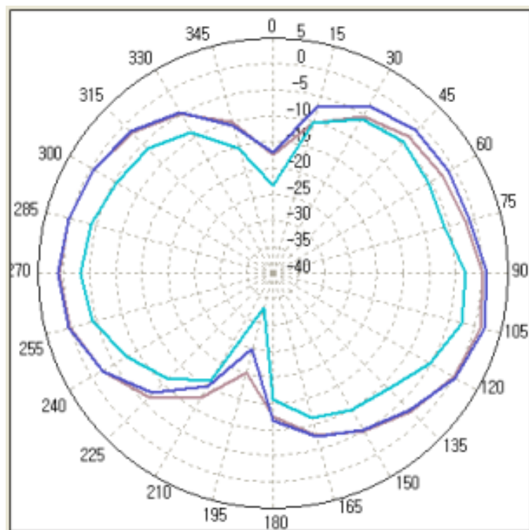
(c) Elevation2 Plane (XZ) – Vertical Polarization
