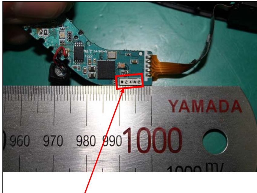
Chip Antenna
