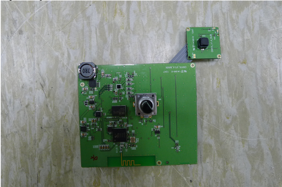
Top view of Main PCB
