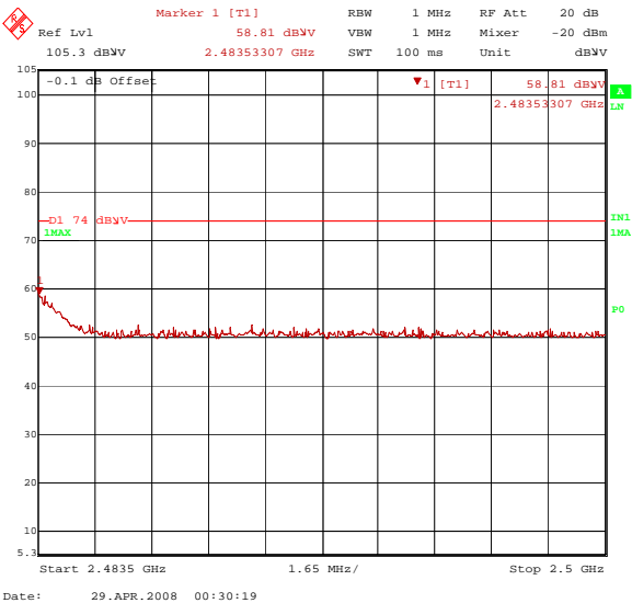
Figure 7. Plot of the Band Edge (Radiated) GFSK Modulation π / 4 DQPSK Modulation Highest Channel (operating at 2480 MHz): PEAK
