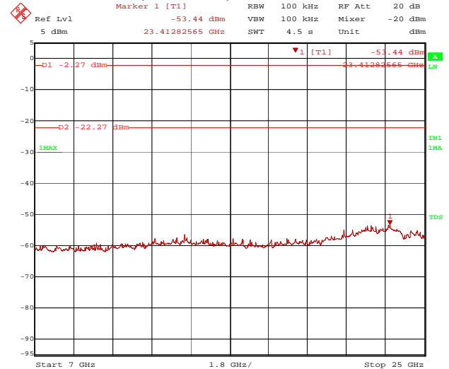
Figure 8: Spurious RF conducted emissions__ \pi/4 DQPSK Modulation
