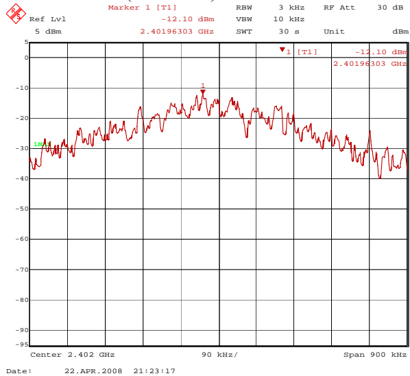
Figure 9. Plot of the Peak Power Spectral Density
