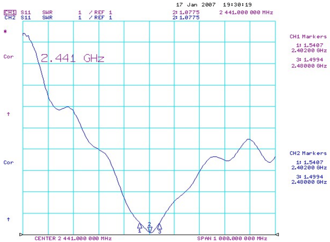
[Picture-1 VSWR]
