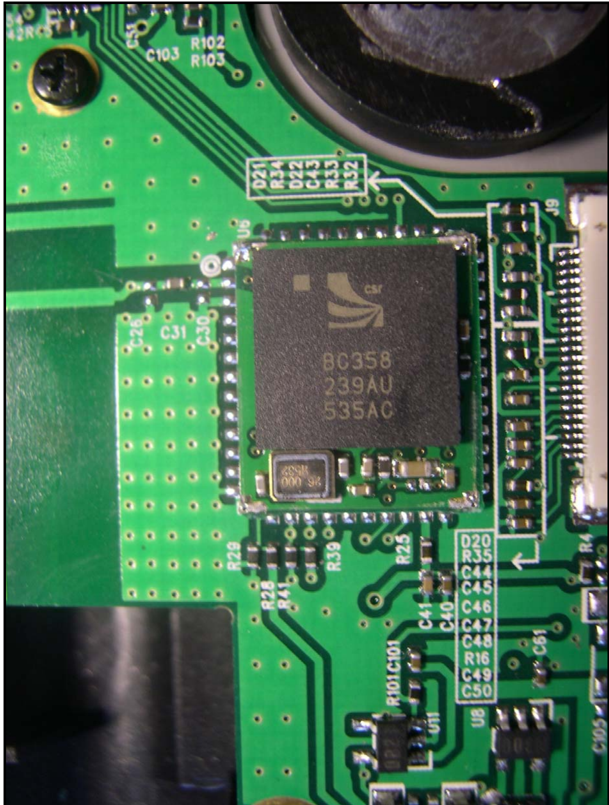
<Photograph 3: View of RF Module within the EUT>
