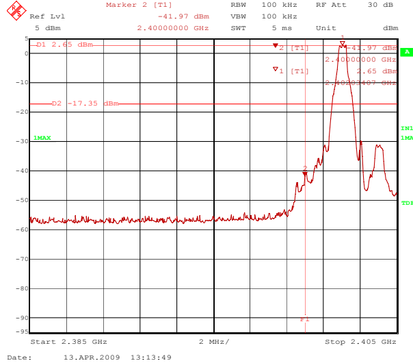
Figure 6. Plot of the Band Edge (Conducted)
