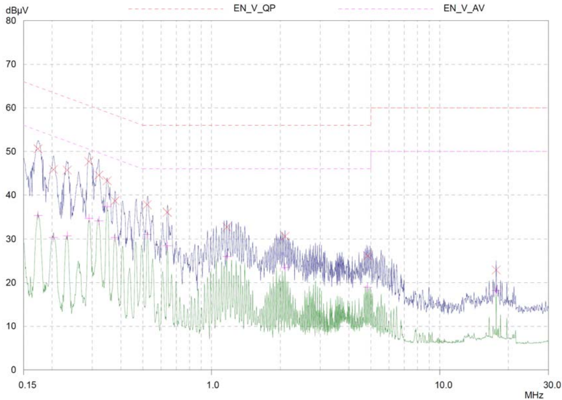
Figure 9. Plot of the AC Power Line Conducted Emissions
