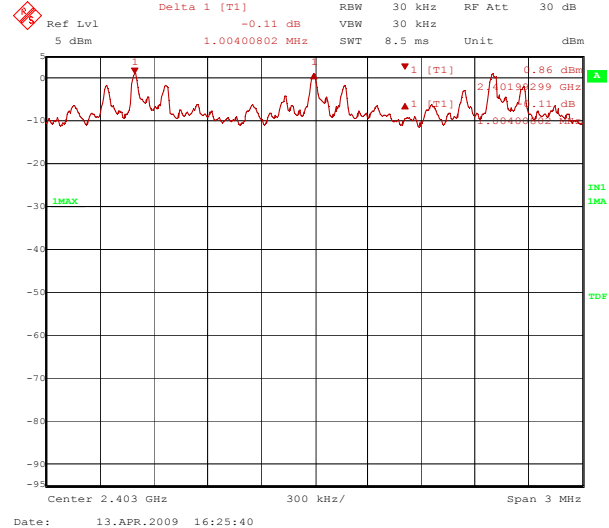
Figure 2. Plot of the Carrier Frequency Separation Basic (GFSK) EDR ( \pi/4 DQPSK)
