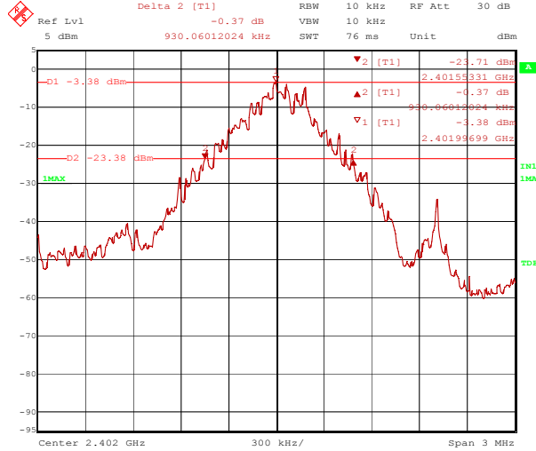
Figure 3. Plot of the 20 dB Channel Bandwidth
