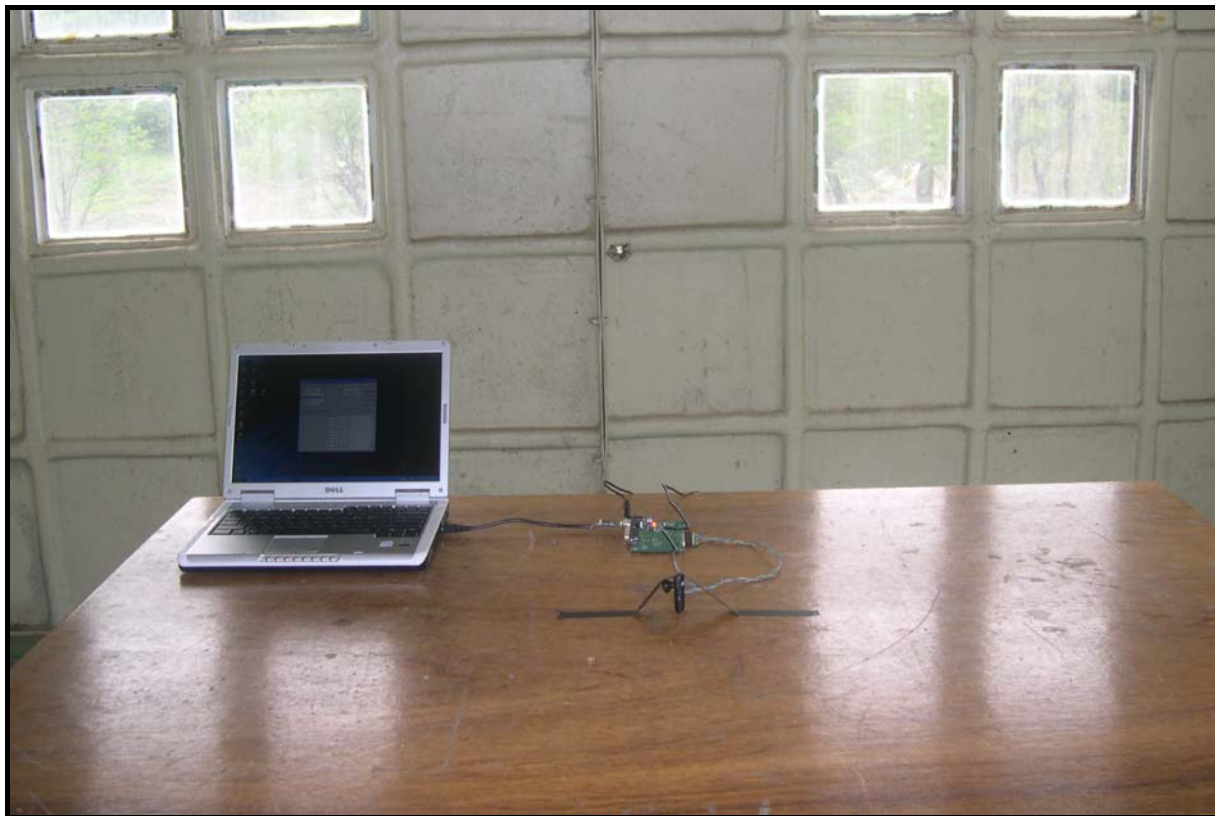
<Radiated Emissions - Rear View>
