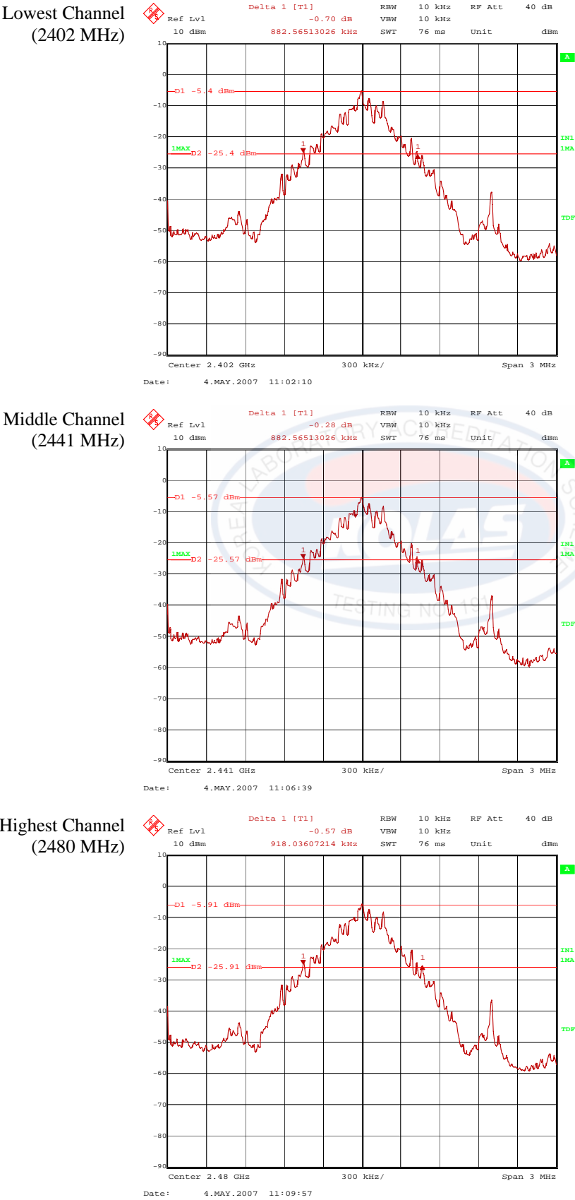
Figure 3. Plot of the 20dB Channel Bandwidth (Conducted)
