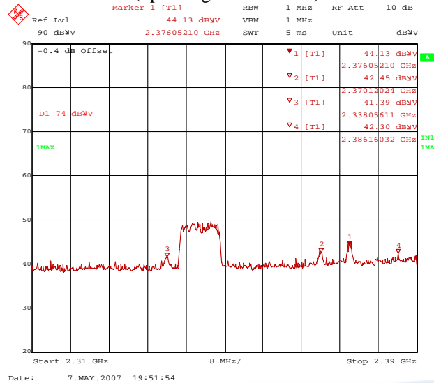
Figure 7. Plot of the Band Edge (Radiated)
