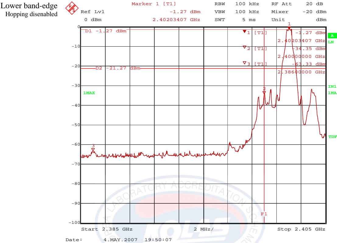
Figure 6. Plot of the Band Edge (Conducted)
