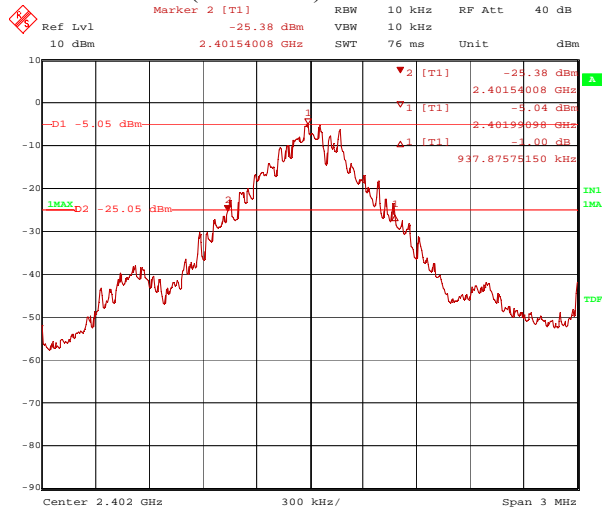
Figure 3. Plot of the 20 dB Channel Bandwidth Basic (GFSK)
