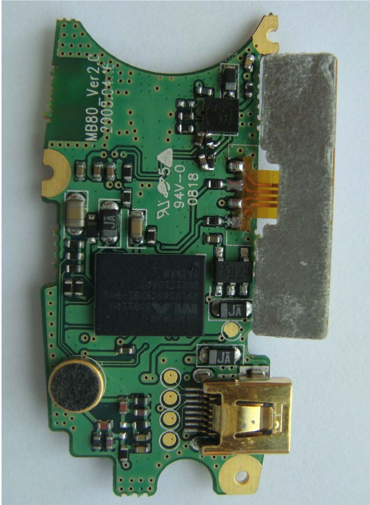
<Photograph 2: Internal Board_ Rear>
